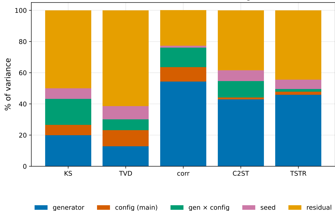
Variance components with generator \times configuration interaction (diabetes, 15 seeds; shared configs)
