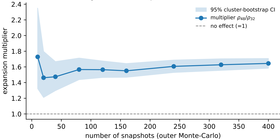
Monte-Carlo convergence of the multiplier
