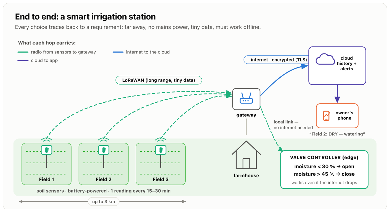
Figure 8.2 — the smart irrigation station, end to end. The watering rule runs locally, not in the cloud.
