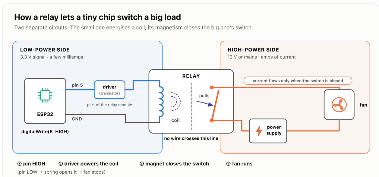
Figure 3.2 — how a relay works. No wire crosses from the small circuit to the big one — magnetism does the switching.
