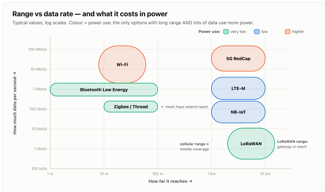
Figure 4.2 — every technology is a trade-off. The only long-range, high-data options use more power.
