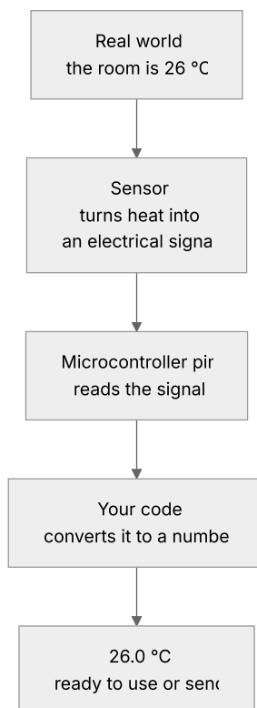
Figure 3.1 — a real-world quantity is turned into an electrical signal by a sensor, read by a pin on the microcontroller, and converted by the code into a meaningful number.
