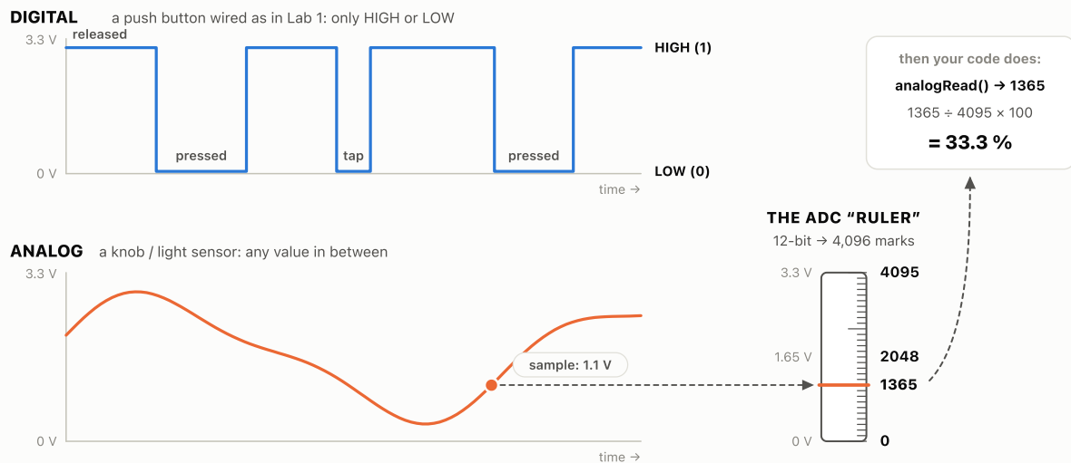
Figure 3.3 — digital vs analog, and how the ADC turns a voltage into a number your code can use.
