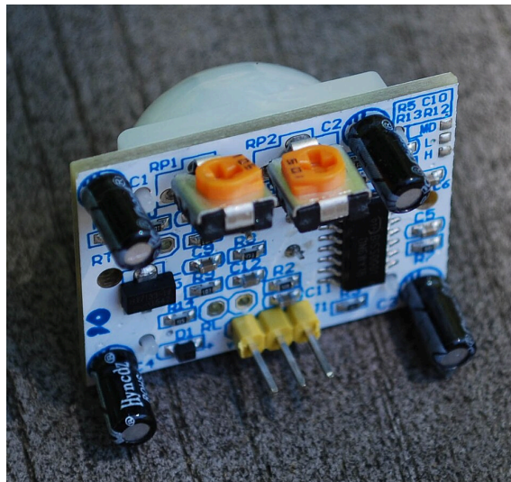
A PIR motion-sensor module. The two orange dials adjust sensitivity and how long it stays on. Photo: Sjilla, CC BY-SA 4.0 , via Wikimedia Commons .
