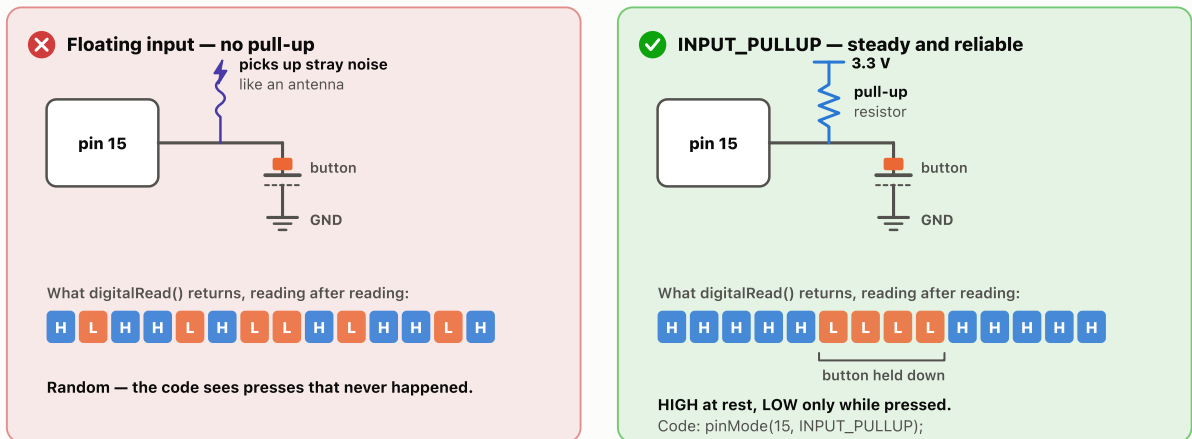
Figure 3.4 — without a pull-up the pin reads noise; with one, it reads HIGH until the button pulls it LOW.
