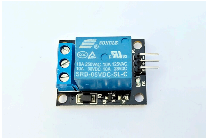
A typical 5 V relay module. The screw terminals connect the high-power circuit. Photo: Suyash Dwivedi, CC BY-SA 4.0 , via Wikimedia Commons .
