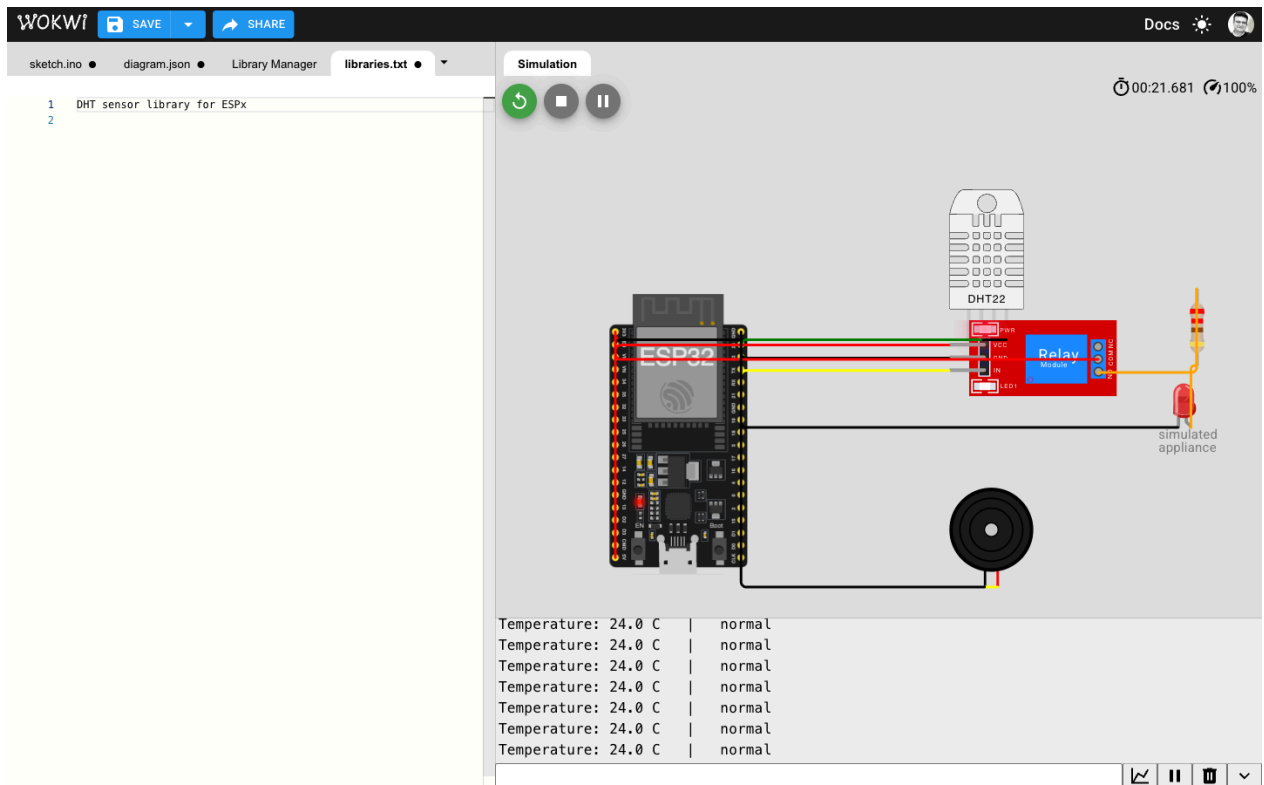
Figure 6.5 — Lab 5 running. Raise the DHT22's temperature above 28 °C and the relay, LED and buzzer switch on by themselves.
