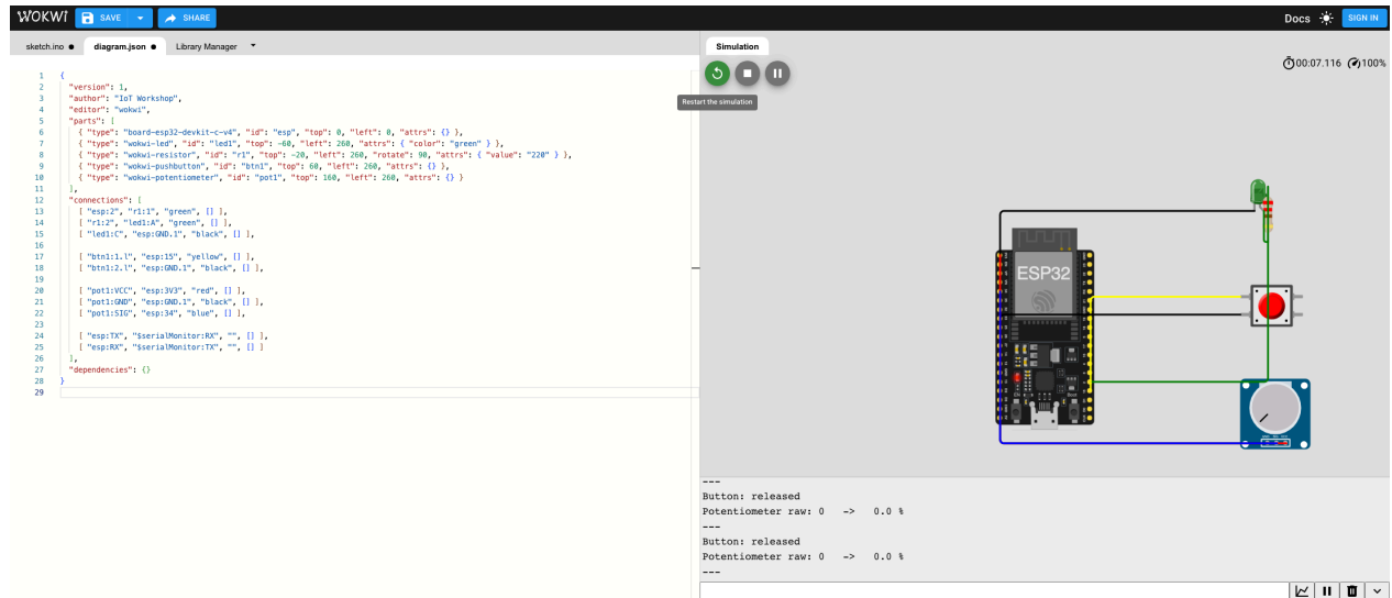
Figure 3.5 — what Lab 1 looks like in the Wokwi simulator: your code on the left, the circuit on the right, and the Serial Monitor underneath.
