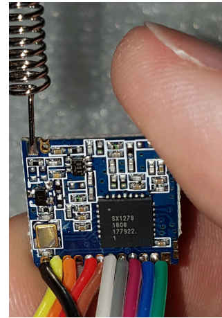
A LoRa radio module — the kind of part inside a battery-powered sensor. (This one is a 433 MHz version; Malaysia's AS923 band needs a module for about 920 MHz.) Photo: Cnd, CC0 , via Wikimedia Commons .
