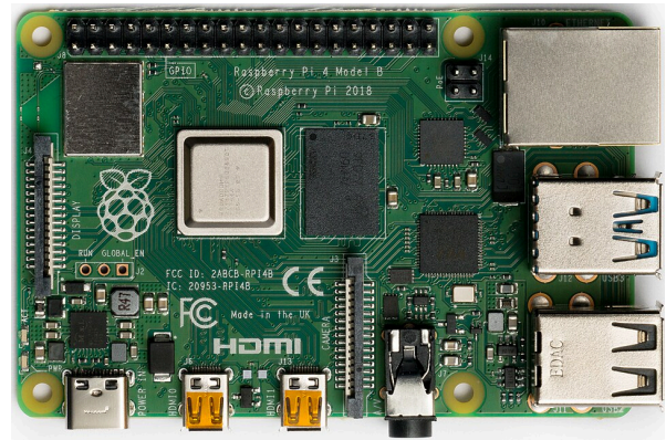
A microprocessor board: the Raspberry Pi 4. Photo: Laserlicht, CC BY-SA 4.0 , via Wikimedia Commons .
