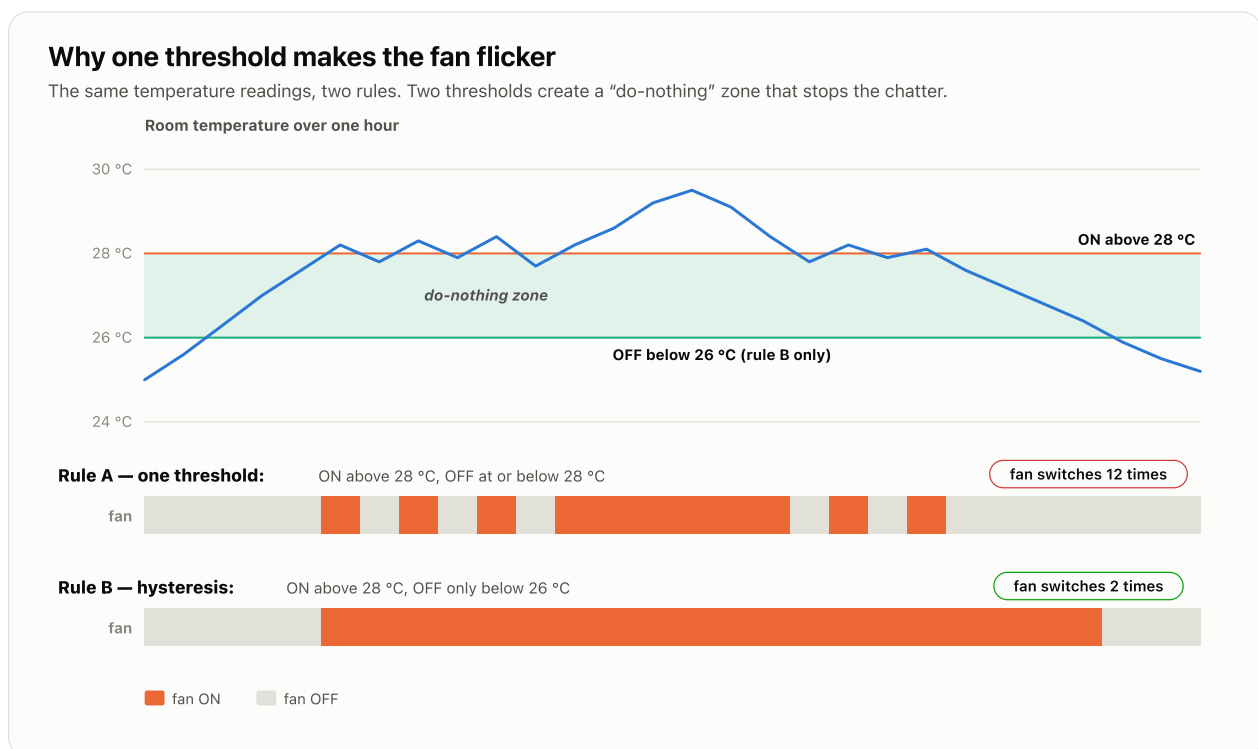
Figure 6.3 — the same readings under two rules. Hysteresis turns 12 annoying switches into 2.
