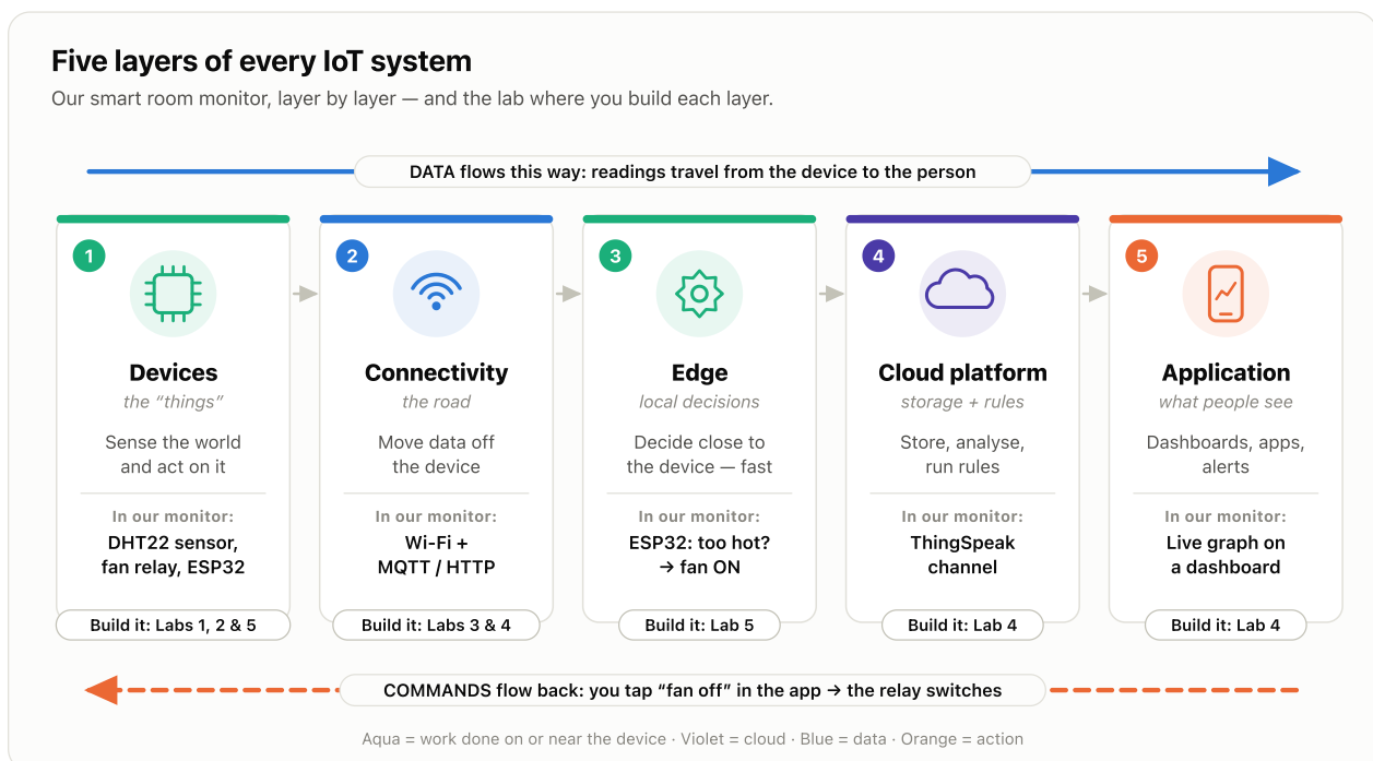
Figure 2.1 — the five layers of our smart room monitor. Data flows towards the person; commands flow back to the device.
