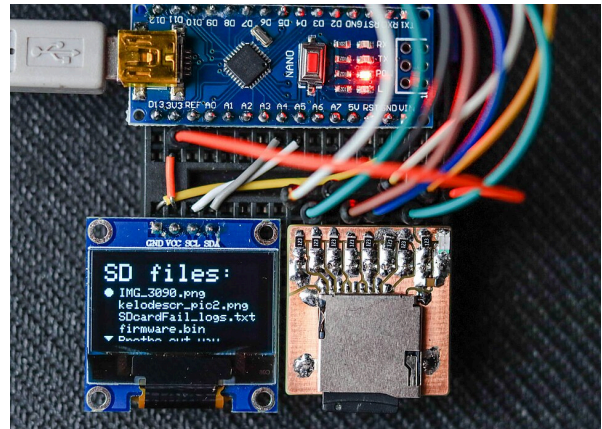
A real breadboard prototype with a small OLED screen, like Lab 6's. Photo: Turbosposk, CC BY-SA 4.0 , via Wikimedia Commons .
