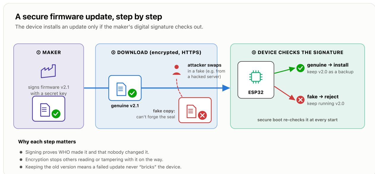
Figure 7.4 — a secure update. The device trusts the signature, not the download.
