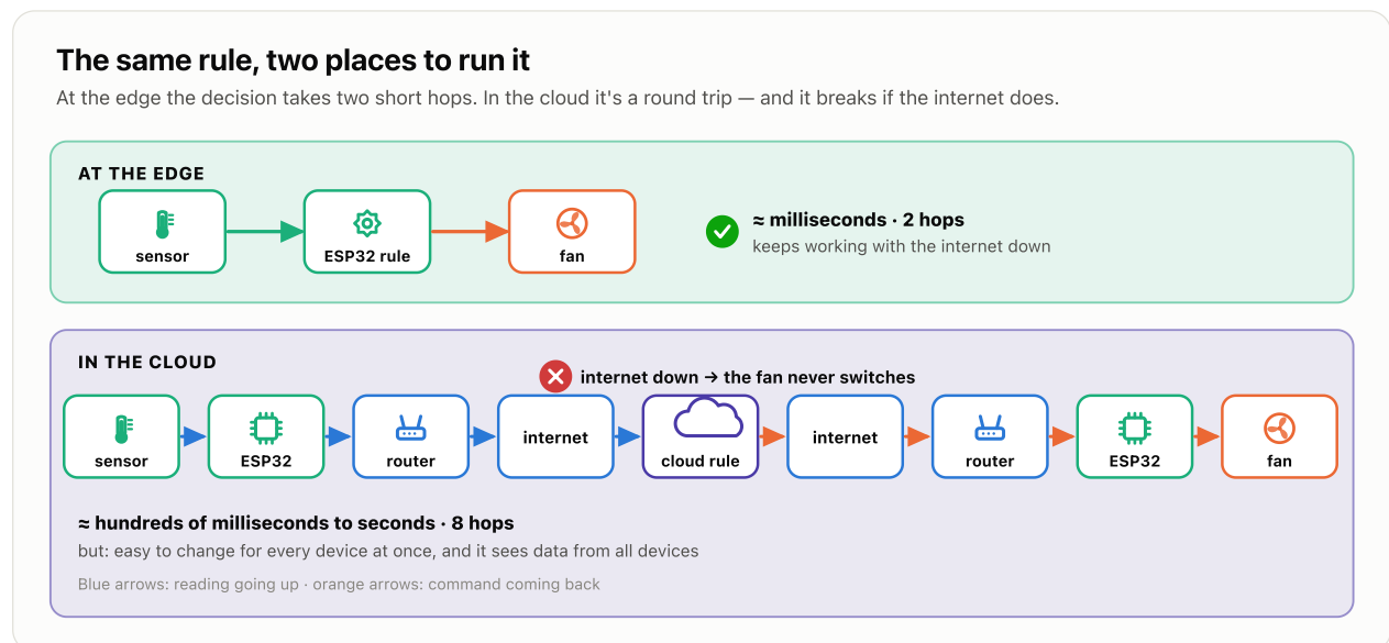
Figure 6.4 — the same rule running in two places. The edge is fast and works offline; the cloud sees every device.
