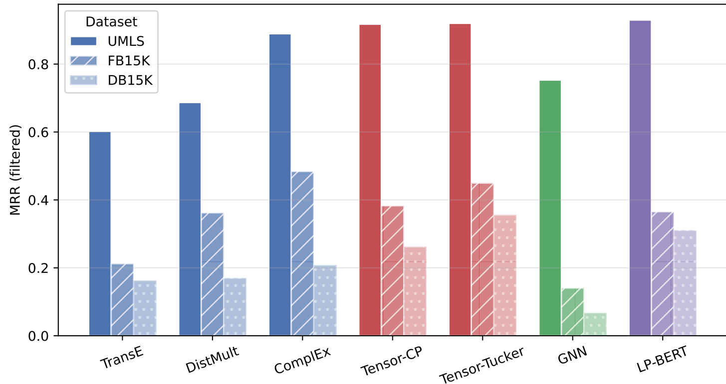
MRR performance comparison across all methods and datasets
