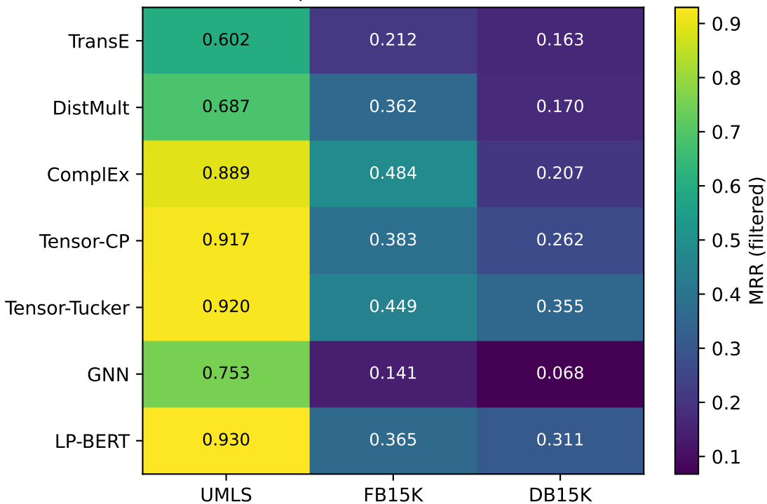
MRR heatmap across models and datasets
