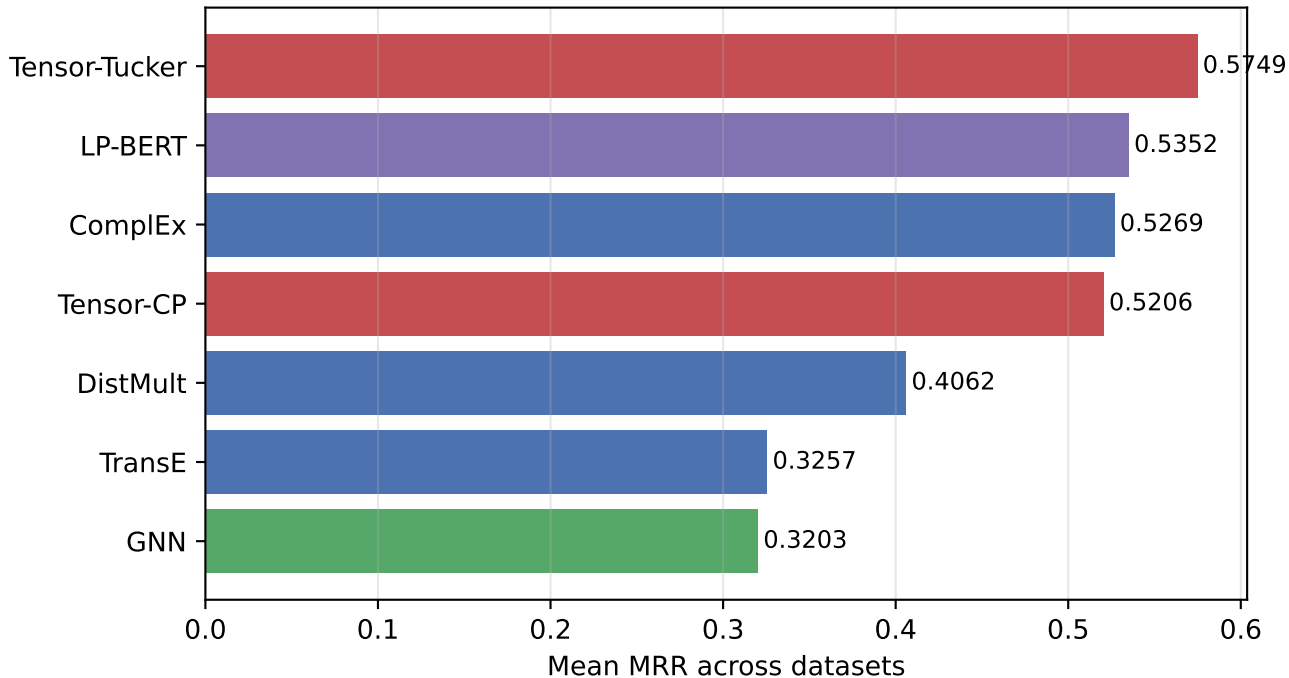
Overall model ranking based on mean MRR
