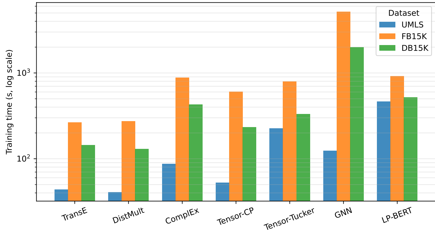
Training time comparison across all evaluated methods
