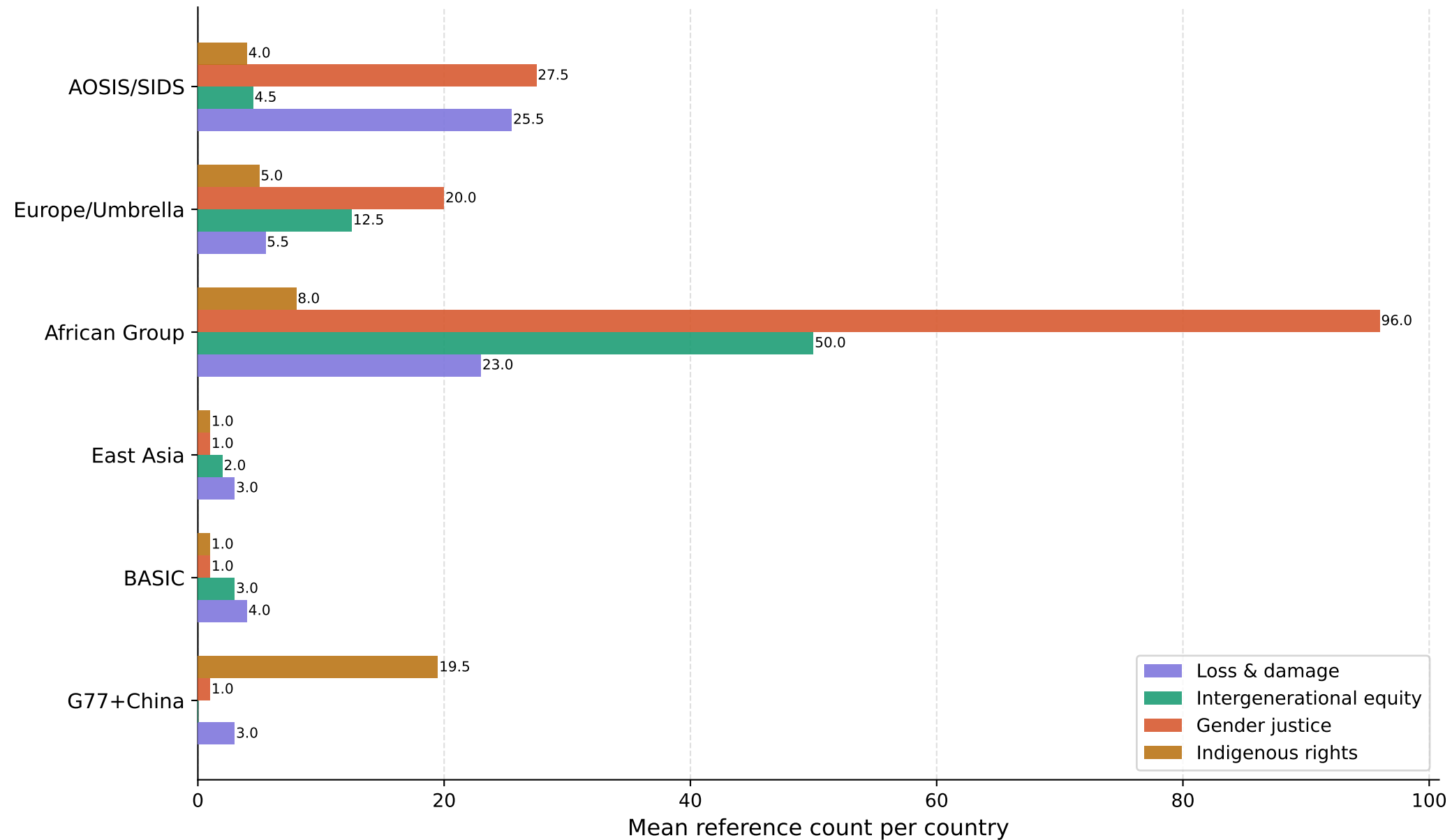
Fig. 5. Climate justice theme frequency in NDCs by UNFCCC negotiating bloc (lexicon tagging on real UNFCCC NDC text; Spearman rho vs GDP = -0.20, p = 0.606)
