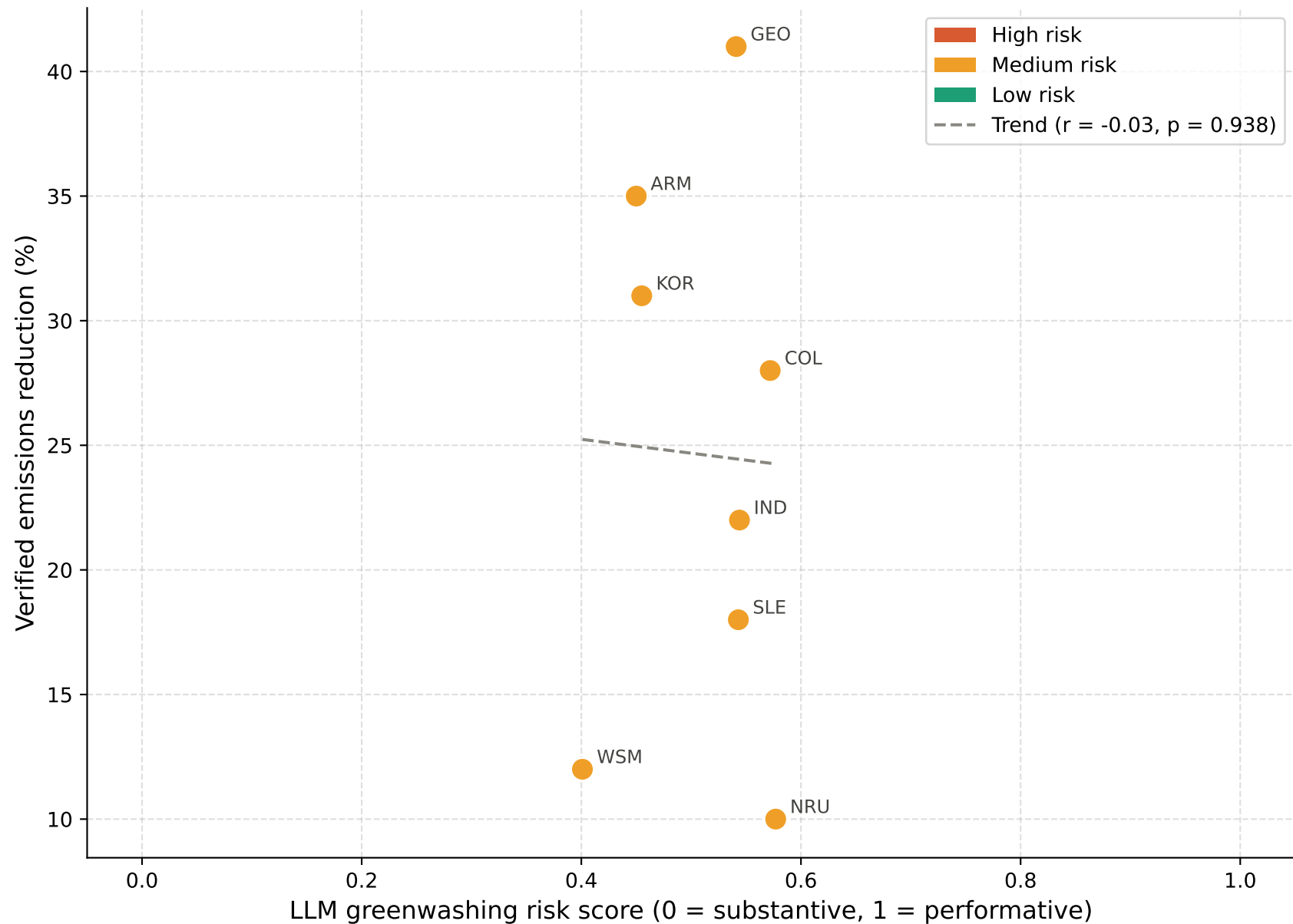
Fig. 4. LLM greenwashing risk score vs. verified emissions reduction (%) by country (real UNFCCC NDC 3.0 documents; Claude scoring; Pearson r = -0.03 )
