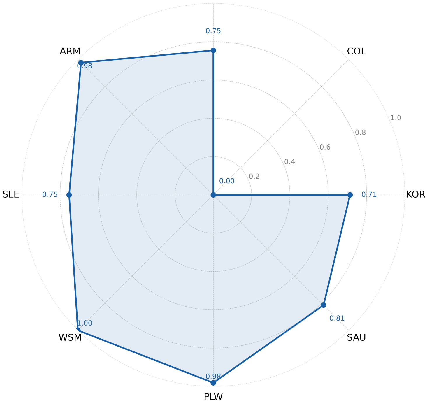
Fig. 2. Semantic similarity to global mean NDC mitigation vector (TF-IDF embeddings on real UNFCCC NDC text, cosine similarity) GEO
