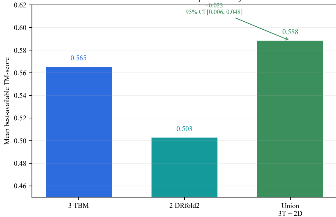
Candidate-bank complementarity
