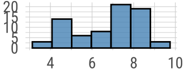
sqrt transformation
