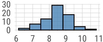
sqrt transformation
