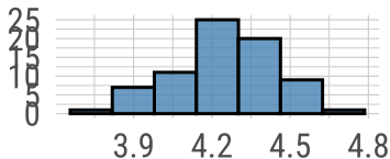
log transformation
