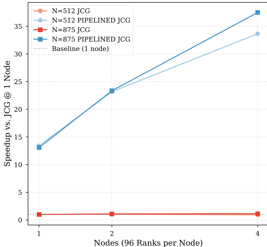
Strong Scaling Speedup (Ref: JCG @ 1 Node)
