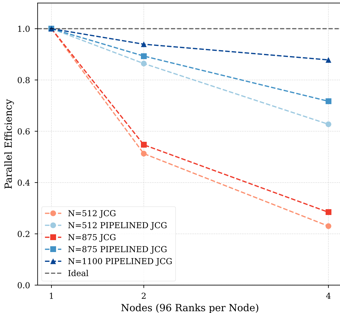
Parallel Efficiency (Ref: Self @ 1 Node)
