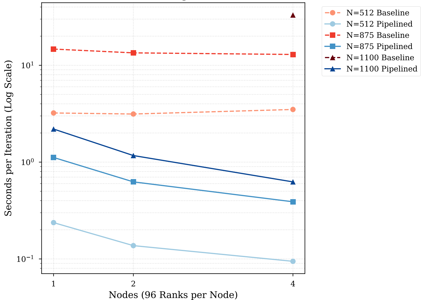
Internode Time per Iteration
