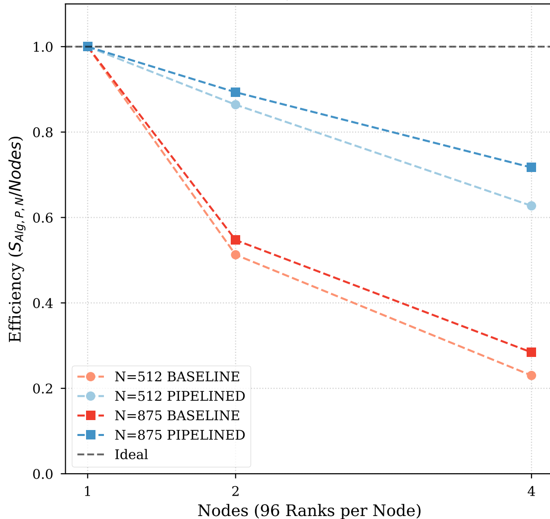
Parallel Efficiency (Ref: Self @ 1 Node)
