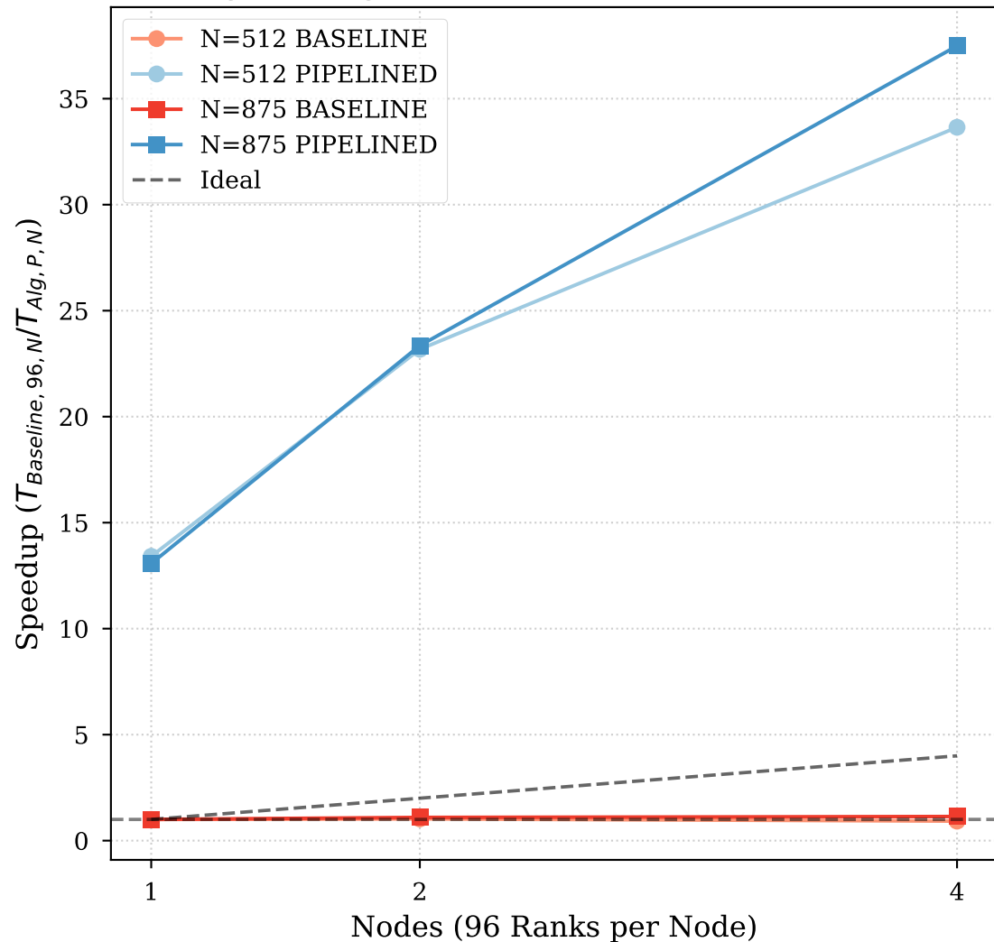
Strong Scaling Speedup (Ref: Baseline @ 1 Node)
