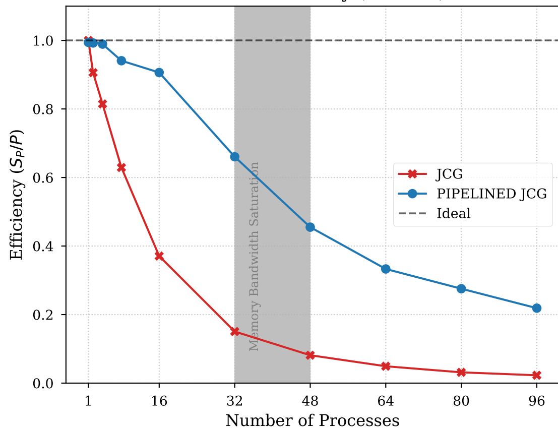
Parallel Efficiency ( N = 400 )
