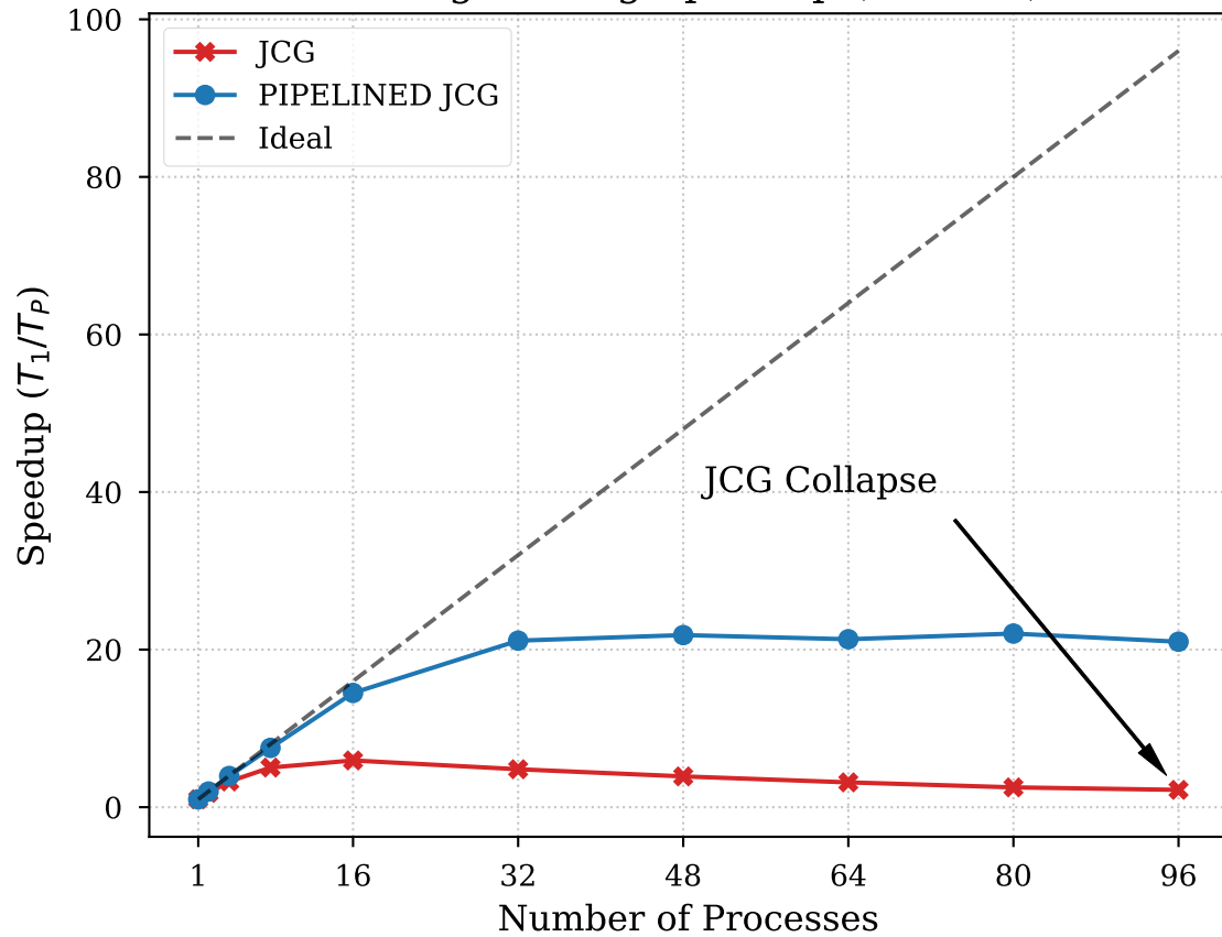
Strong Scaling Speedup ( N = 400 )
