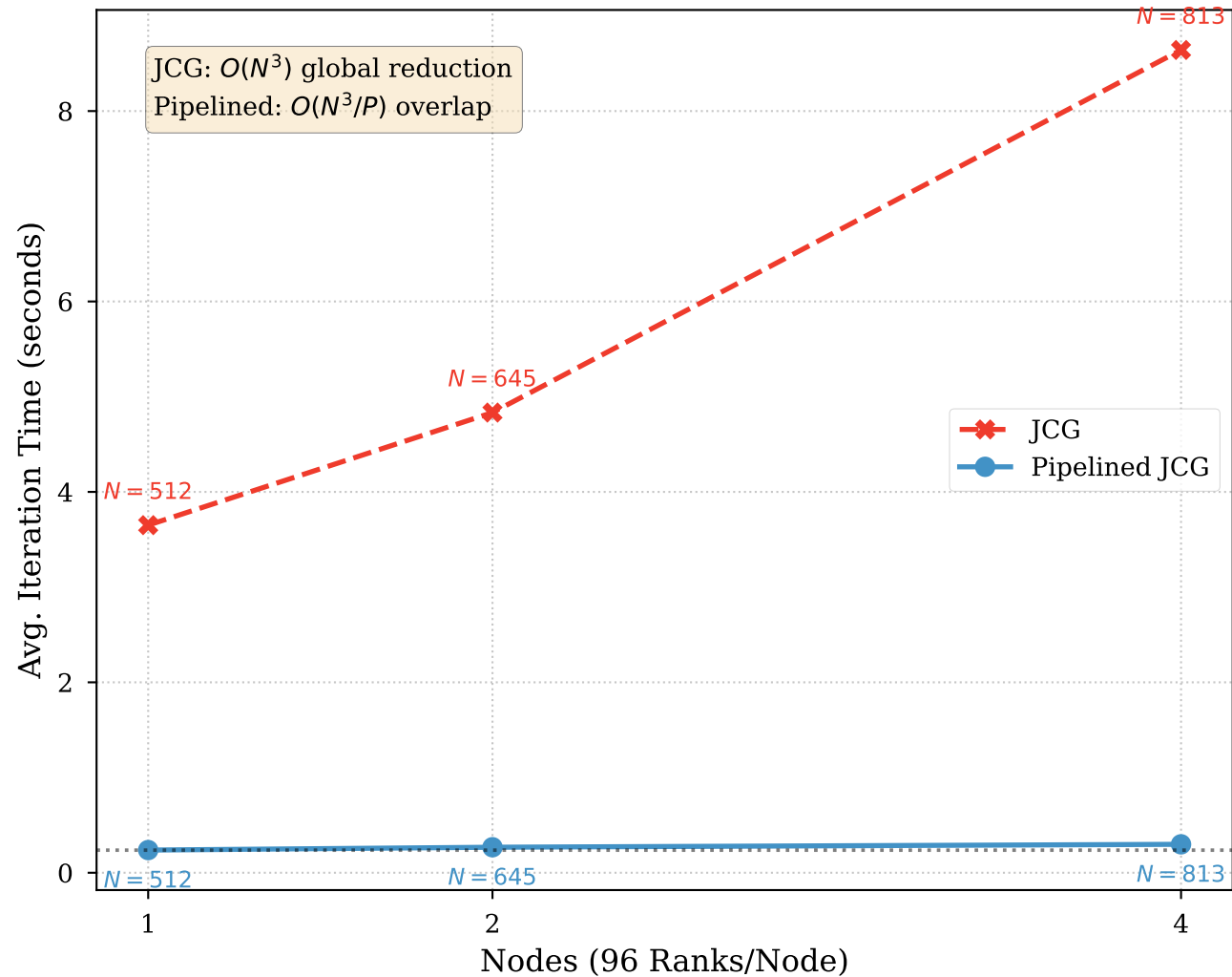
Weak Scaling: Avg. Iteration Time
