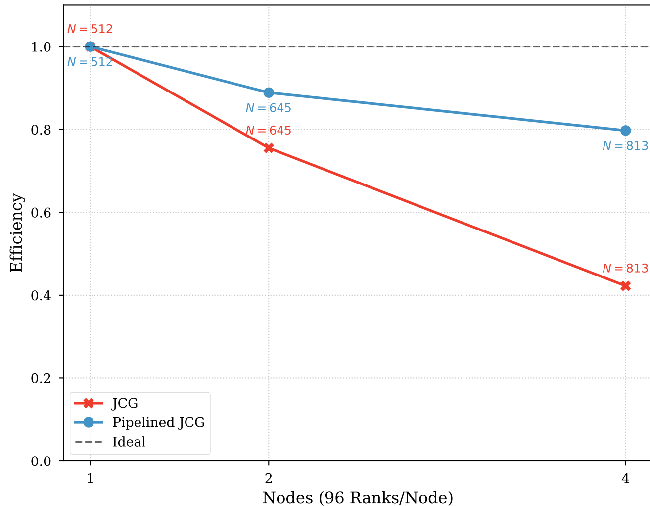
Weak Scaling Efficiency
