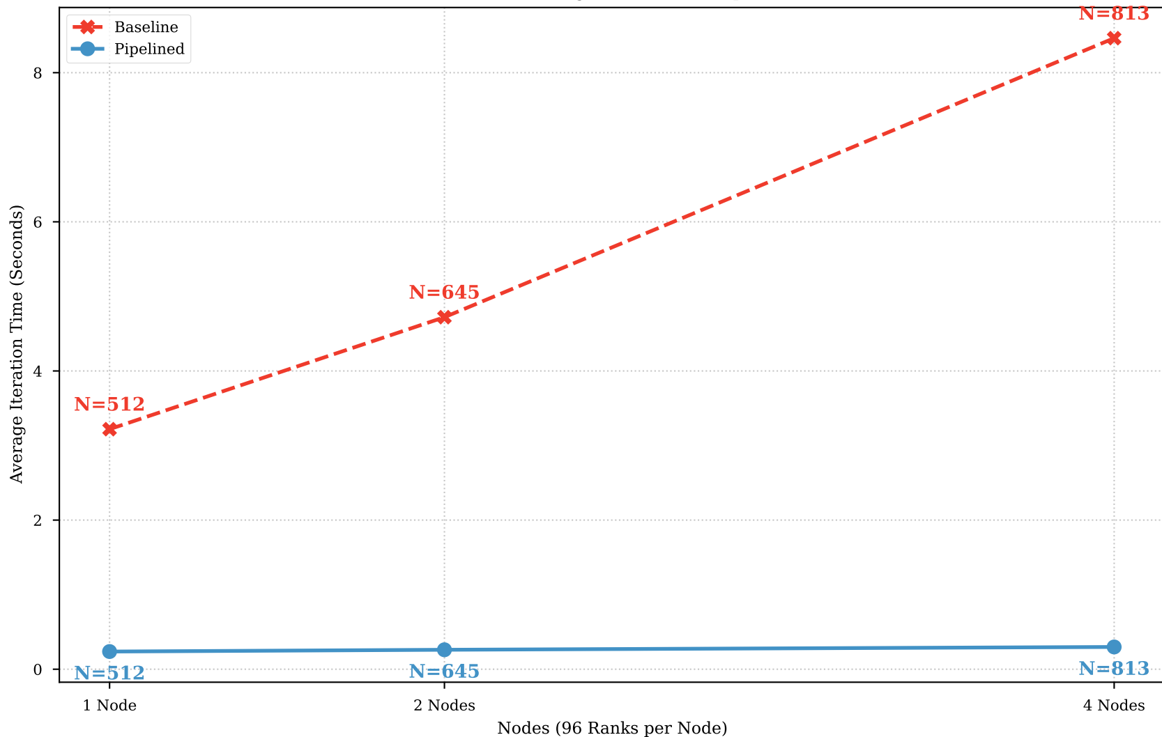
Internode Weak Scaling: Iteration Time per Grid Size
