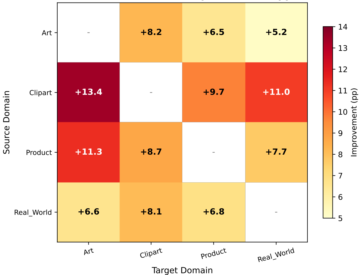
Office-Home: CDAN Adaptation Gain (pp)
