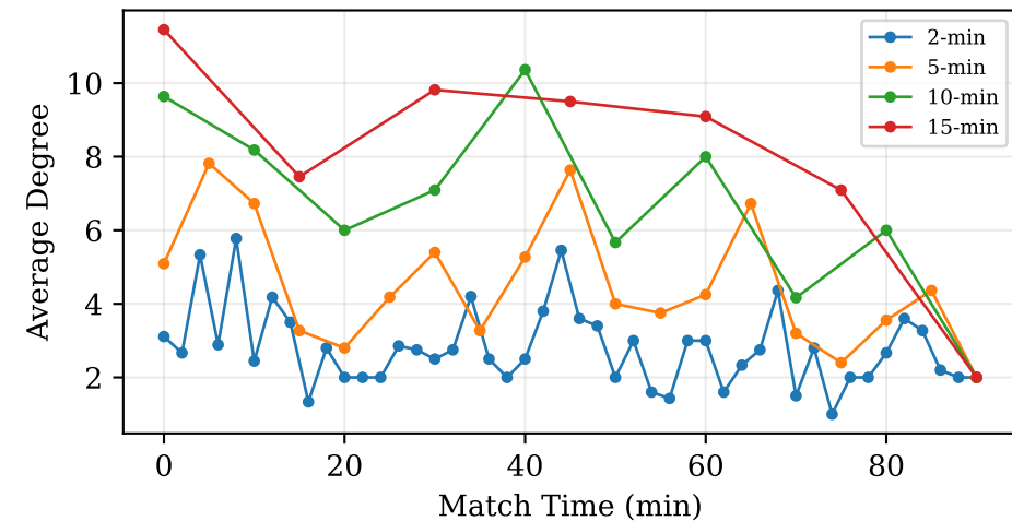
Average Degree
