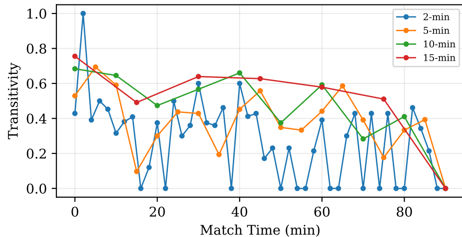
Transitivity
