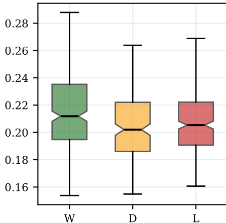
Network Density (H=18.5, ***)
