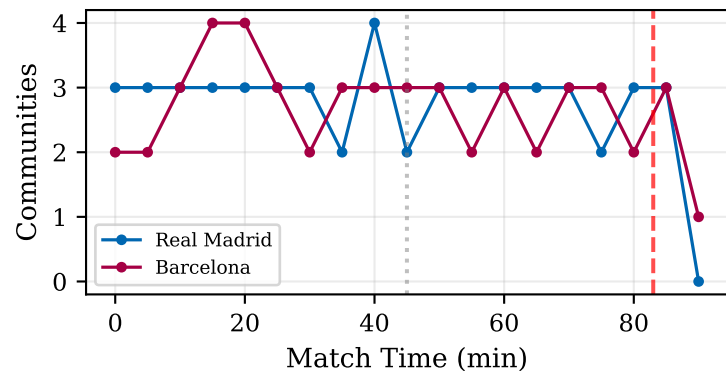
(f) Number of Communities
