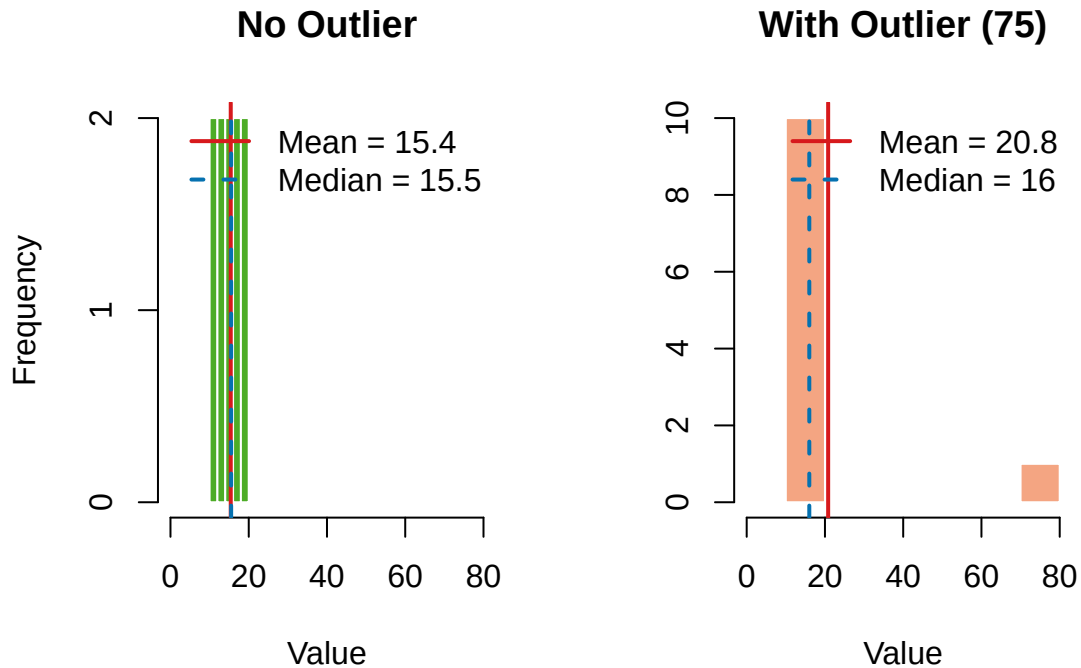
Figure 10.1.: Effect of outliers on mean vs median.
