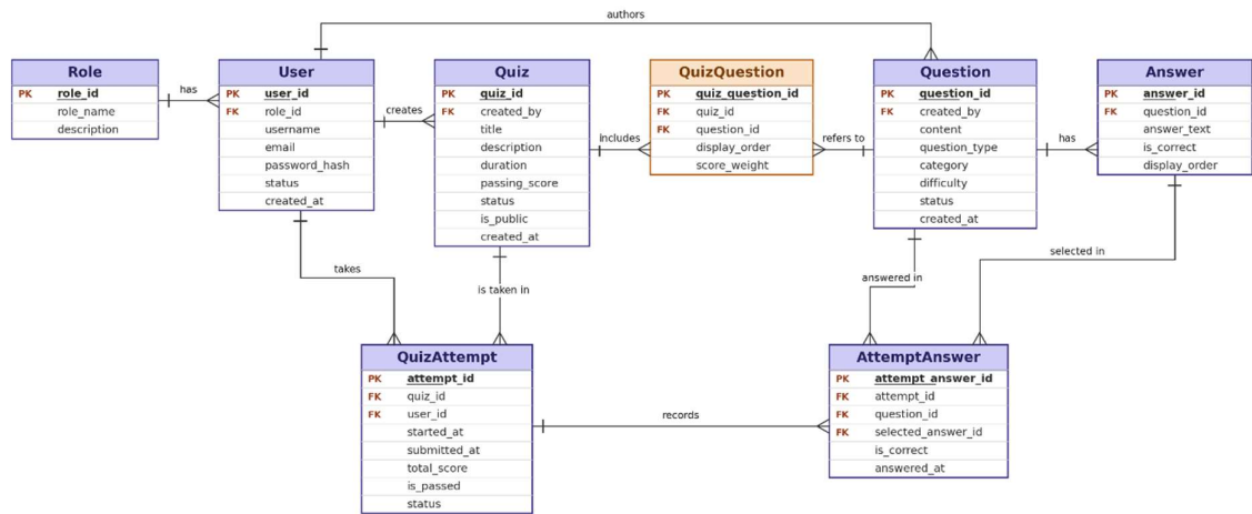
Figure 8: Entity Relationship Diagram
