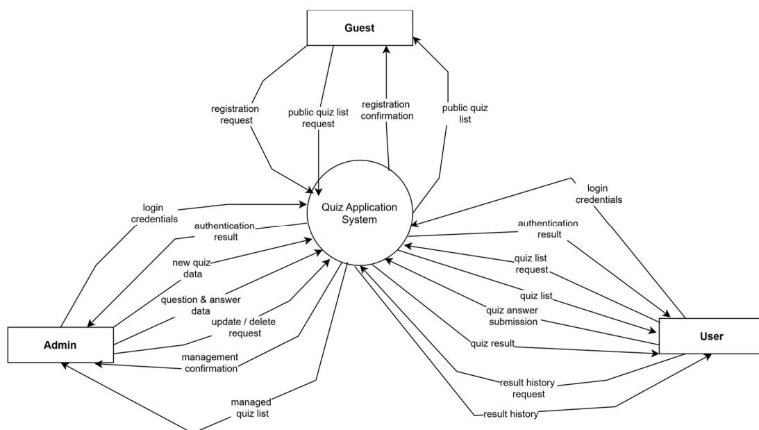
Figure 1: Context Diagram of Quiz Application System
