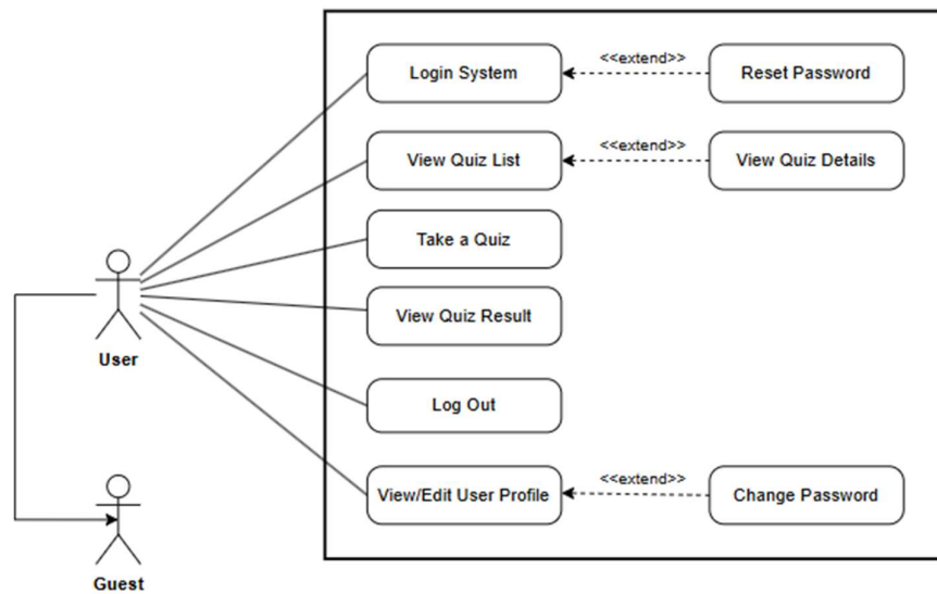
Figure 6: UCs for User
