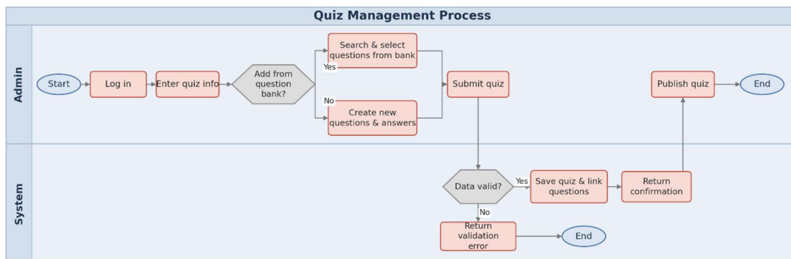
Figure 3: Quiz Management Process Diagram
