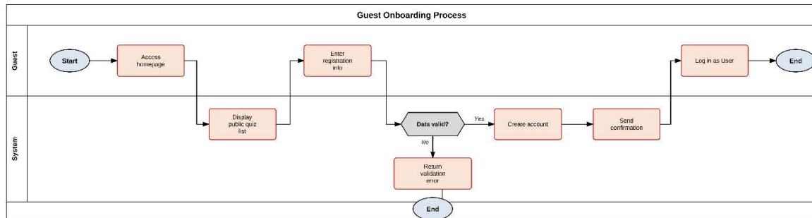
Figure 4: Guest Onboarding Process Diagram
