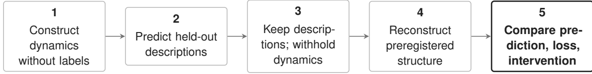
Figure 7. The core protocol. The label firewall between stages 2 and 3 prevents reverse reconstruction from using the original dynamics. Targets, distances, model classes, and thresholds are preregistered.
