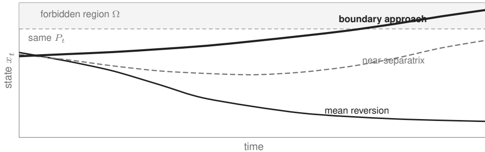
Figure 6. Synthetic positive-control geometry. Episodes with the same coarse description occupy different dynamical regimes and have different reachable futures. The trajectories illustrate the preregistered construction; confirmatory values are generated from the declared system family rather than inferred from this schematic.
