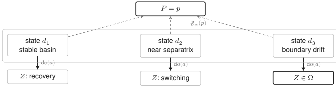
Figure 5. Intervention-sensitive psychological fibre. Three states support the same description yet the same intervention produces different futures. The fibre diameter measures this within-description divergence; the example is schematic.
