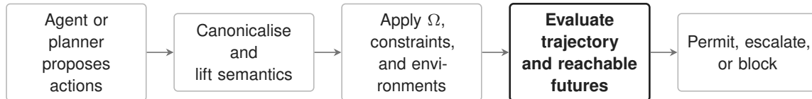
Figure 8. Runtime Governance at the execution boundary. The system governs a proposed action trajectory before tools run. Its safety claims remain scoped to the represented environment, policy, horizon, and tested failure modes.
