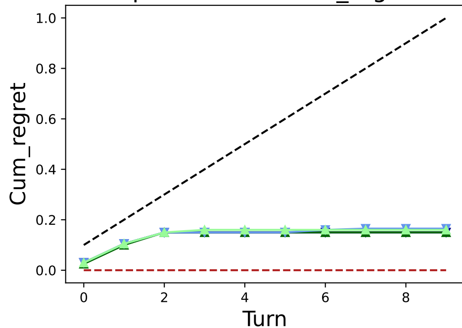
Alphanumeric Cum_regret
