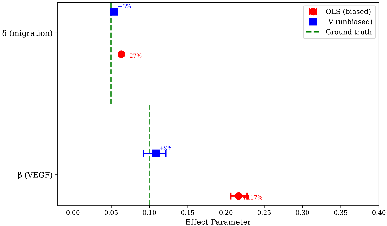
Causal Effect Estimates: OLS vs. Instrumental Variable
