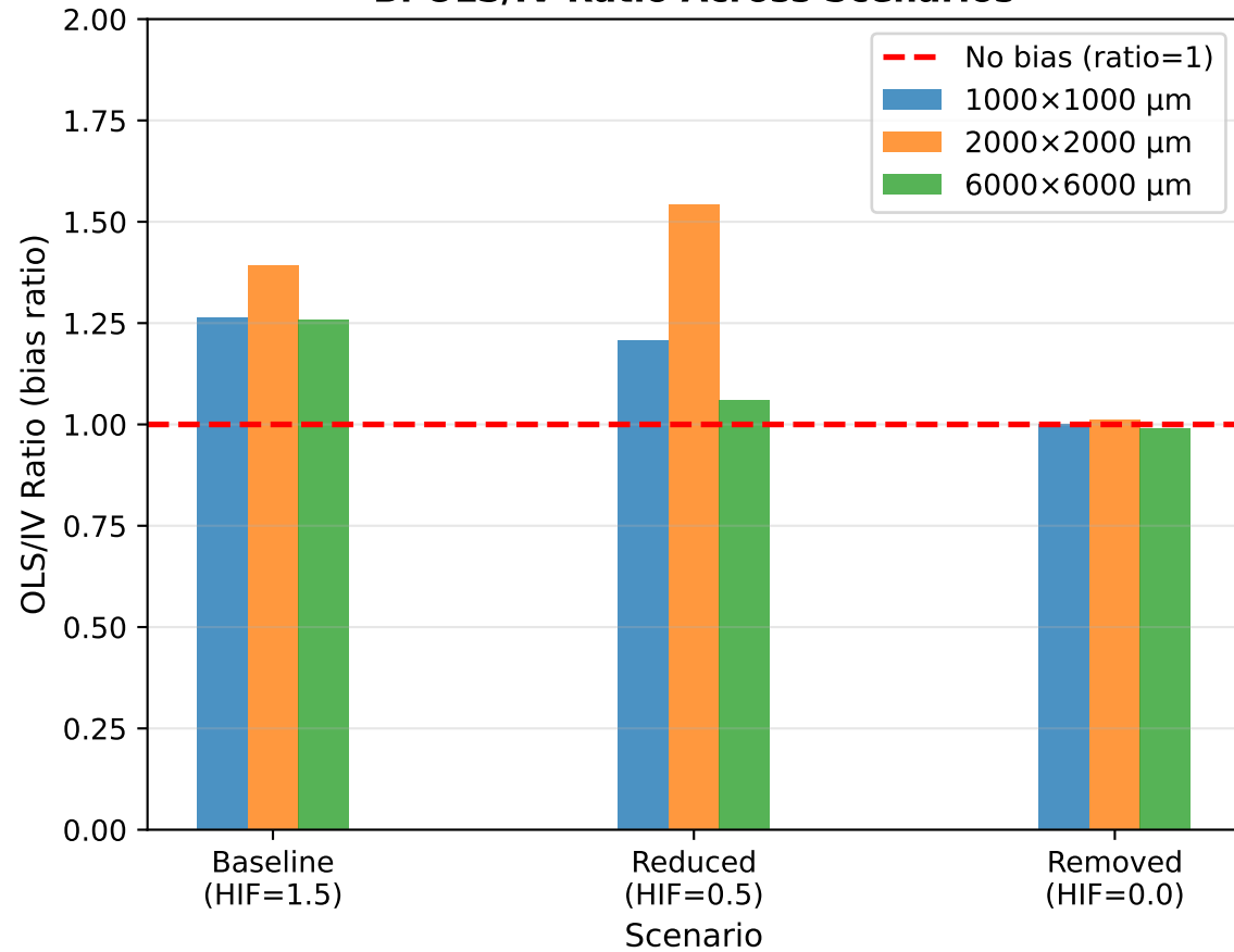
B. OLS/IV Ratio Across Scenarios
