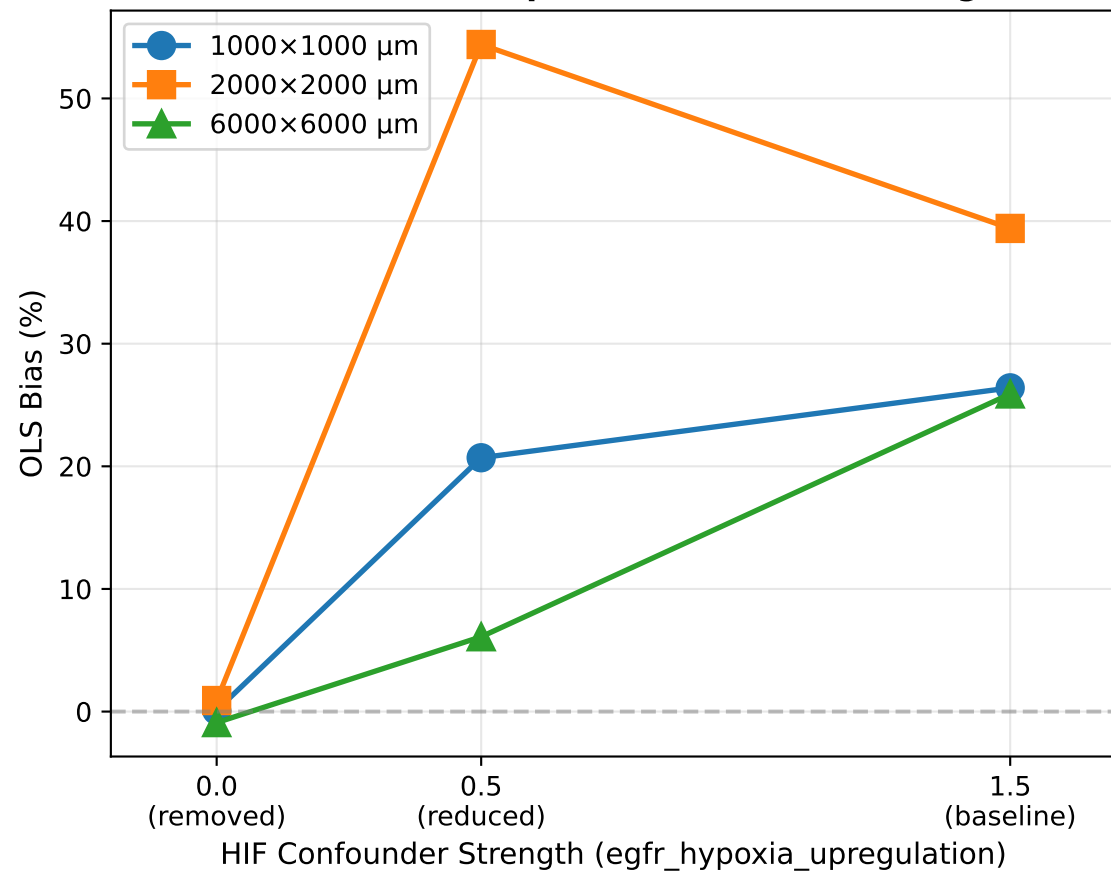
A. OLS Bias Proportional to Confounding
