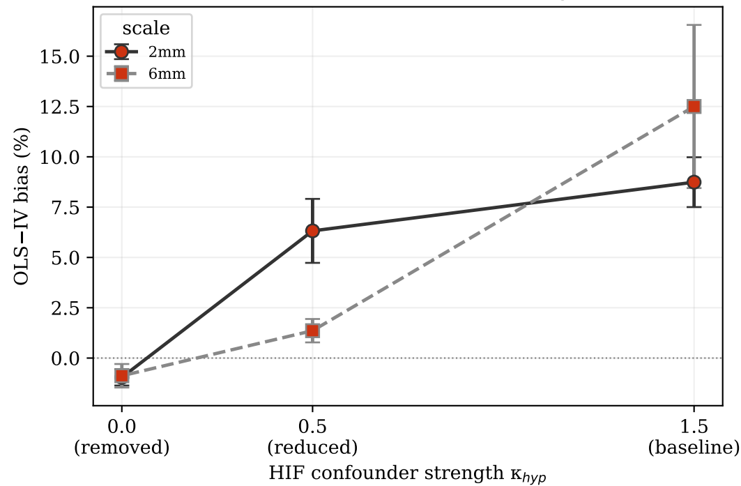
A. OLS bias collapses when confounding removed
