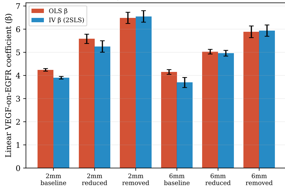
B. OLS-IV gap narrows as HIF decreases
