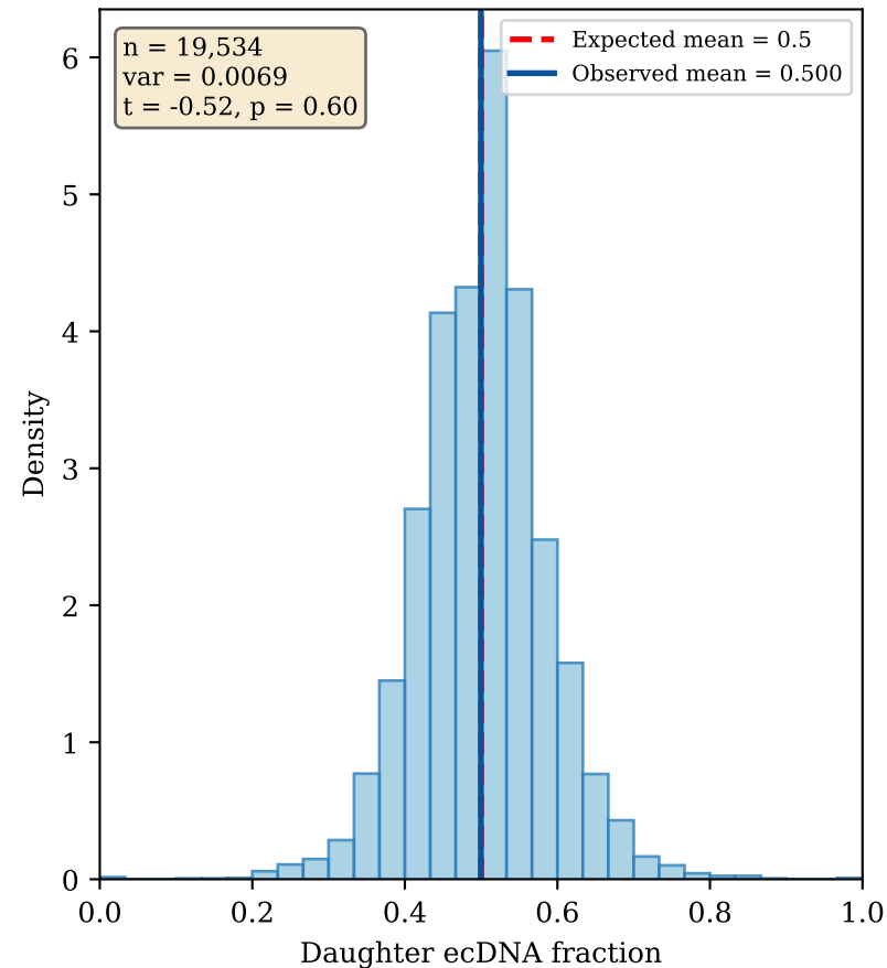
A. ecDNA segregation distribution
