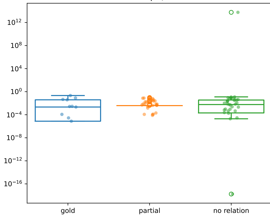
ShapIQ
