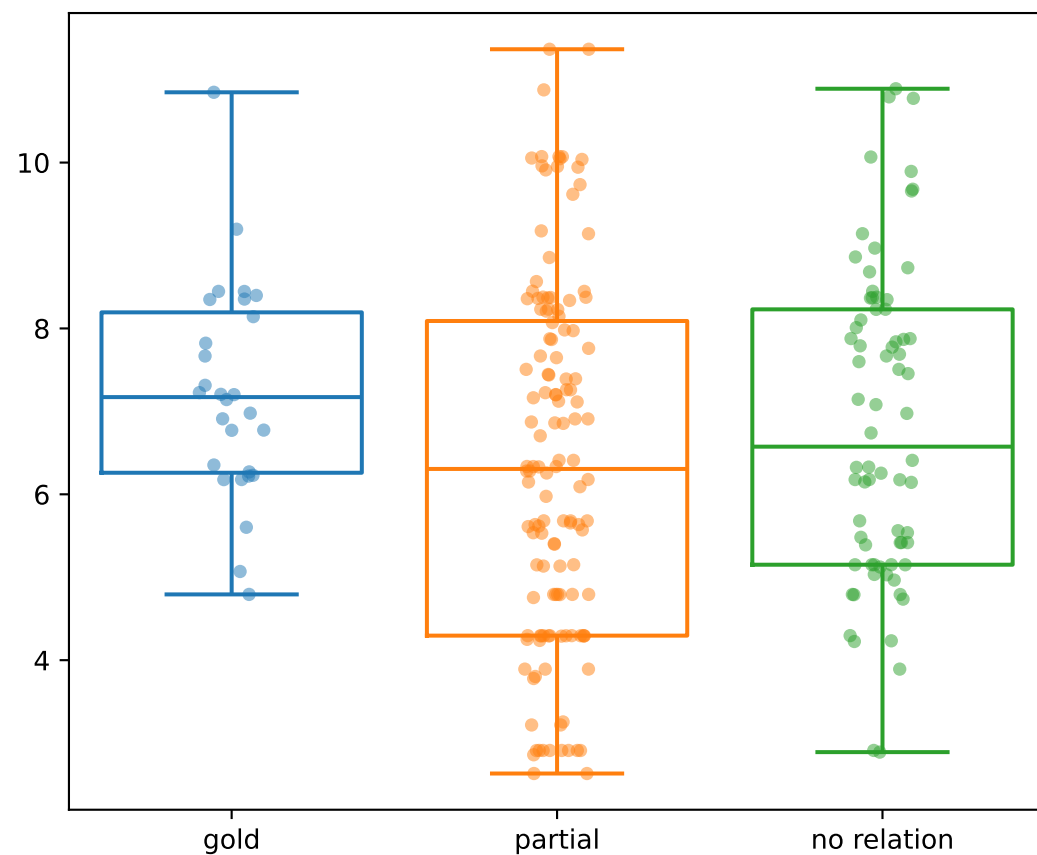
ShapIQ
