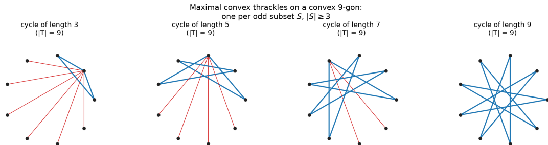
Figure 2: One maximal convex thrackle for each odd subset size m of a convex 9-gon: the cycle C_S in blue, the forced pendant edges in red. Theorem 4.4 says there is exactly one for each such S , and |E| = 9 always.
