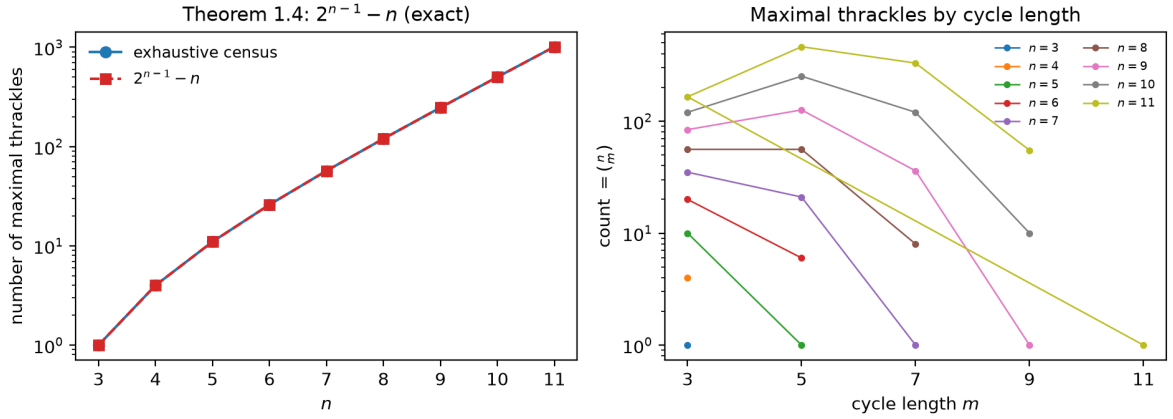
Figure 1: Left: the number of maximal convex thrackles against n , together with the closed form 2^{n-1} - n (logarithmic scale). Right: the number of maximal thrackles of cycle length m , which is exactly \binom{n}{m} for every odd m \geq 3 and every n tested.
