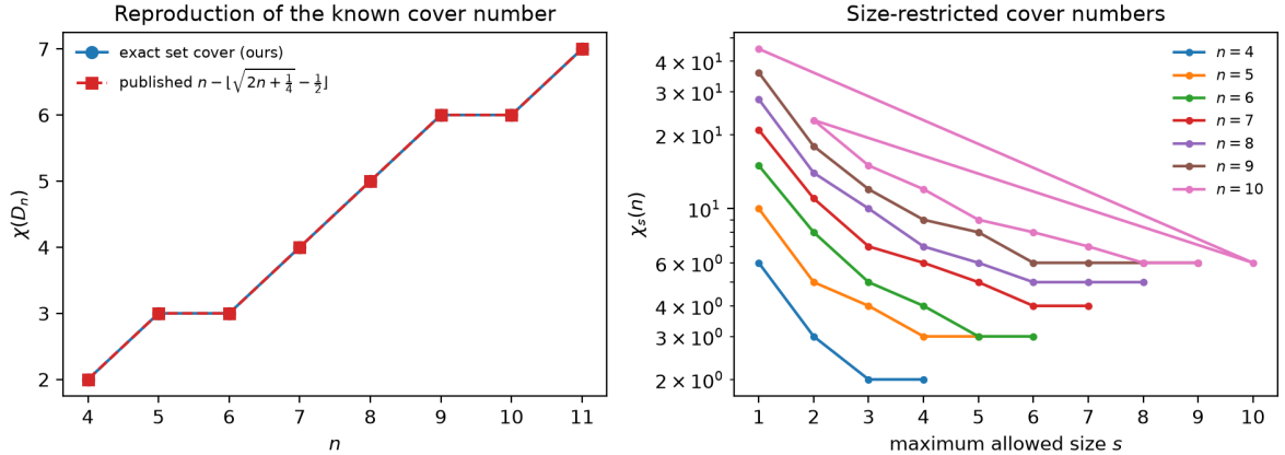
Figure 4: Left: the cover number \chi(D_n) computed by integer programming against the published closed form. Right: the size-restricted numbers \chi_s(n) for s = 1, \dots, n and n \leq 10 ; for s = n the value is \chi(D_n) .
