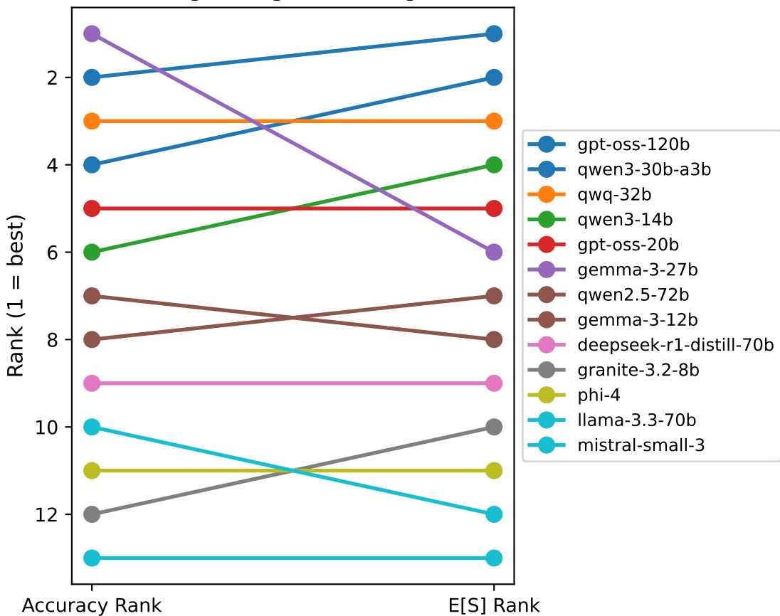
Ranking Divergence — Legal NLI
