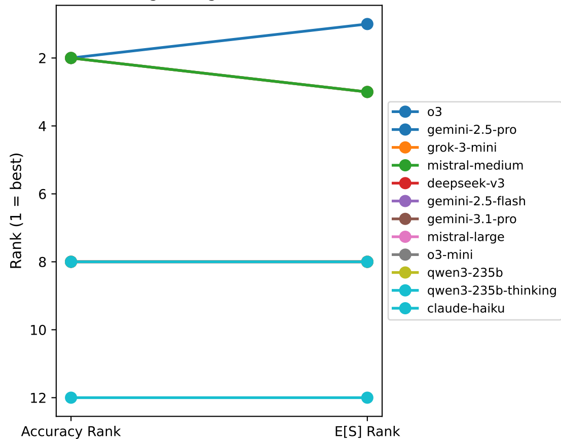
Ranking Divergence — Finance
