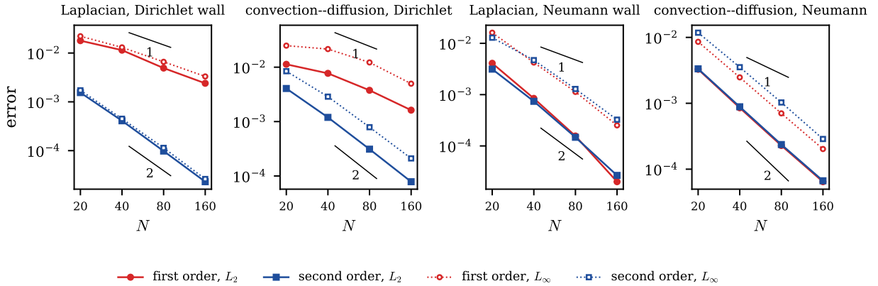
Figure 13: Manufactured problems with the OpenFOAM operators ( ibmOrderTest ): L_2 and L_\infty errors with the first-order treatment (V0/F0) and the second-order treatment (V1/F1); convection uses the face-centre value (C0) in both.
