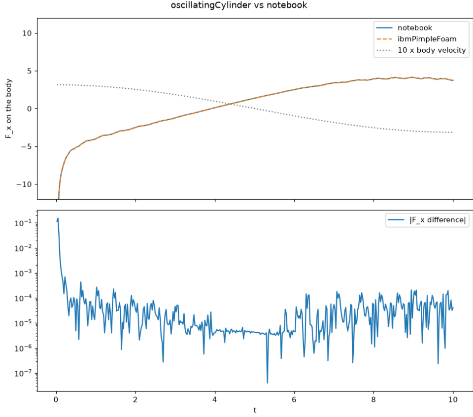
Figure 8: Oscillating cylinder: streamwise force on the body against the reference (top) and their difference (bottom).
