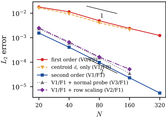
Laplacian, Dirichlet wall
