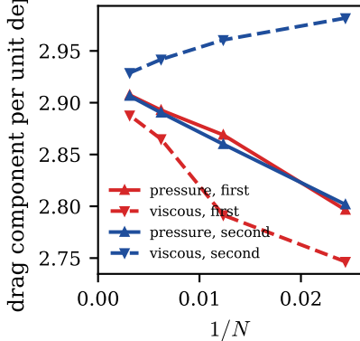
(b) no slip, components
