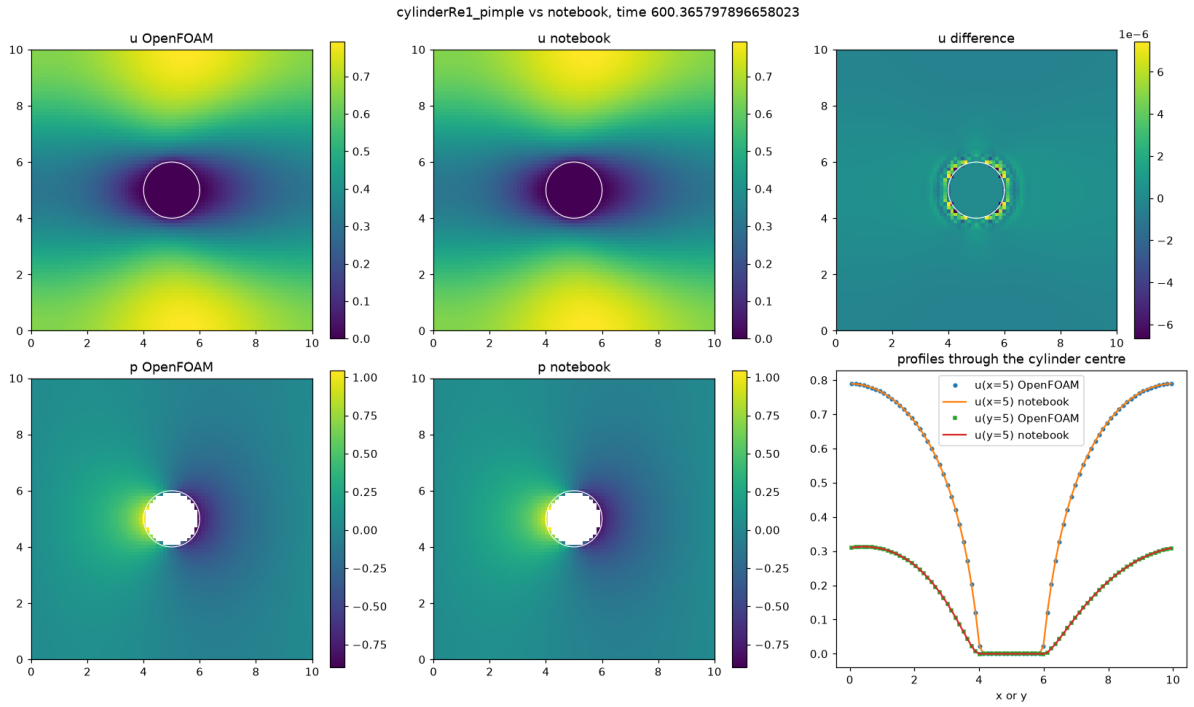
Figure 6: Body at rest, transient solver with the reference's pseudo-time step: streamwise velocity (top) and pressure (bottom) against the reference, difference field, and profiles through the cylinder centre.
