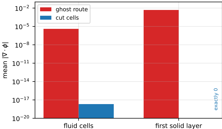
Continuity error, 45-degree free-slip channel
