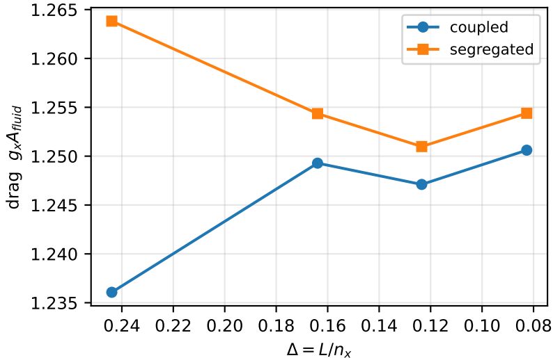
Free-slip cylinder, Re_R = 1.25 , upwind ghost
