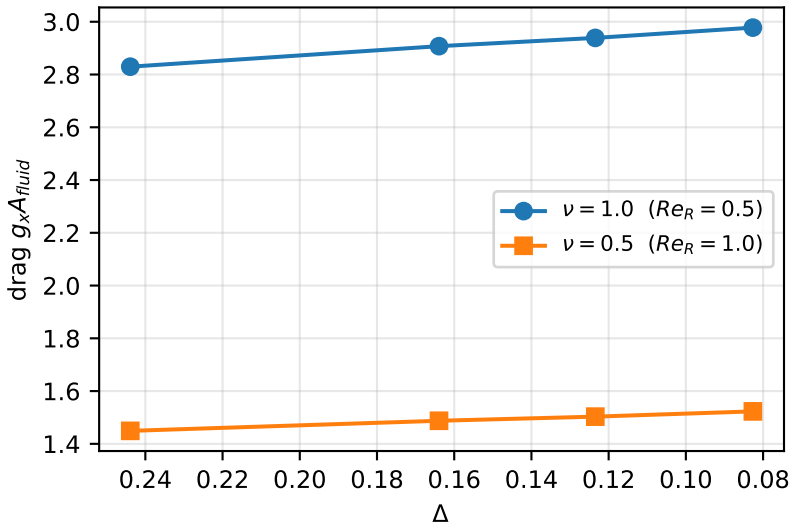
Cut-cell route, free-slip cylinder
