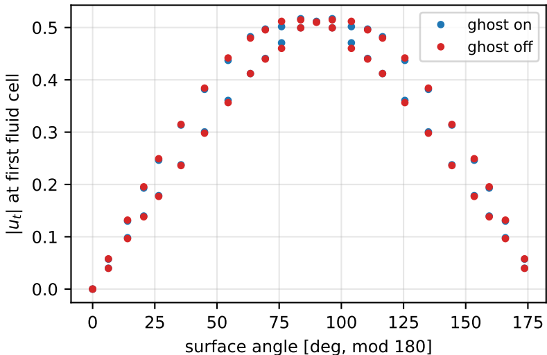
Tangential slip around the cylinder
