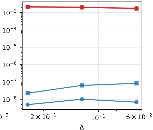
|g_x| (exact: 0)
