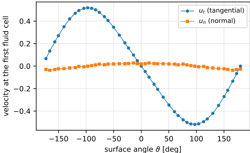
Slip and penetration around the cylinder
