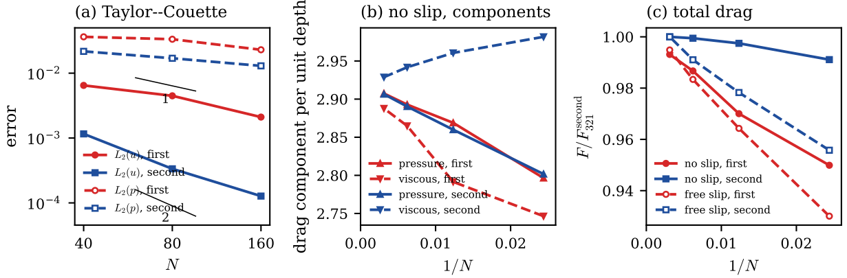
Figure 15: Coupled problems. (a) Taylor–Couette flow: L_2 errors of velocity and pressure. (b) No-slip cylinder at Re_D = 1 : pressure and viscous drag. (c) Total drag of the no-slip and free-slip cylinder relative to the second-order value at N = 321 .
