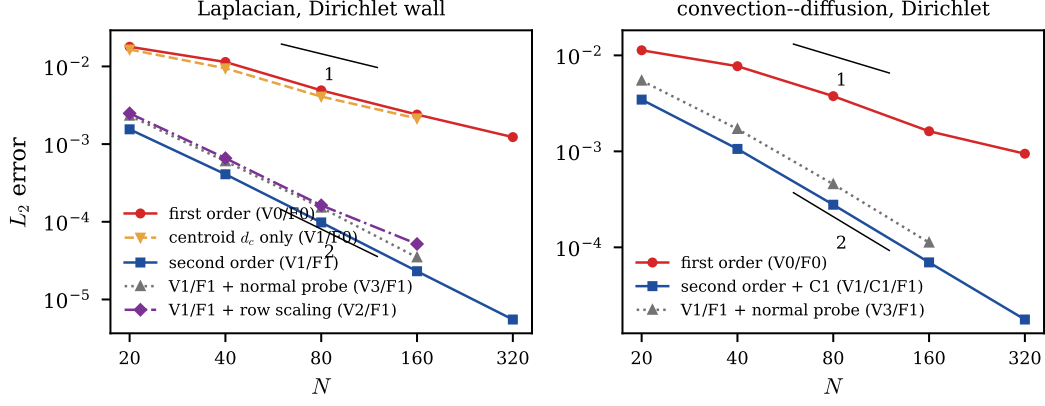
Figure 14: Ablation of the ingredients on the Dirichlet problems (Python implementation, up to N = 320 ): V0/V1 wall distance (7)/(37); F0/F1 face flux of cell centres / (34); V2 row scaling with the cell Laplacian; V3 three-point normal probe; C1 convective value at the wet-face centroid.
