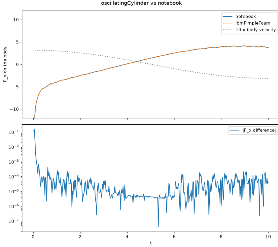
Figure 7: Oscillating cylinder: streamwise force on the body against the reference (top) and their difference (bottom).
