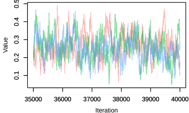
Trace – mean.p
