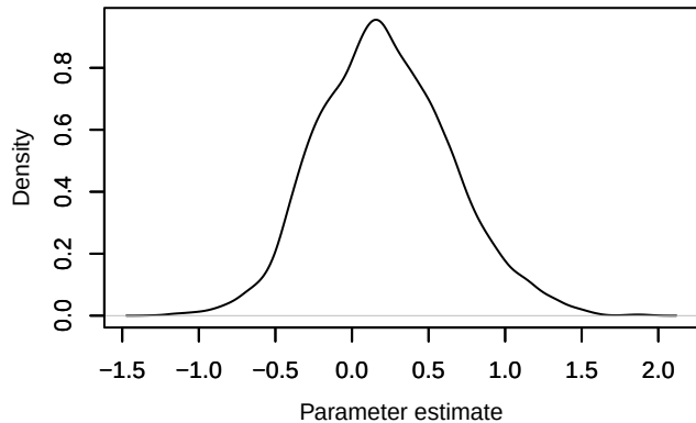
Density – betaISLAND_a[4]
