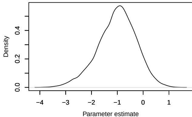
Density – betaISLAND_a[3]
