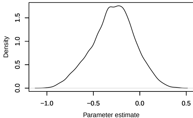
Density – betaSEX[2]
