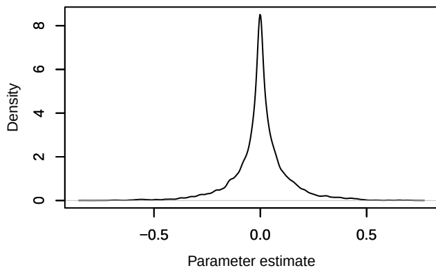
Density – betaISLAND_b[5]
