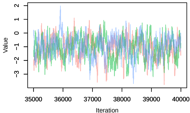
Trace – betaISLAND_b[1]
