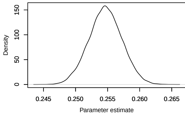
Density – mean.p
