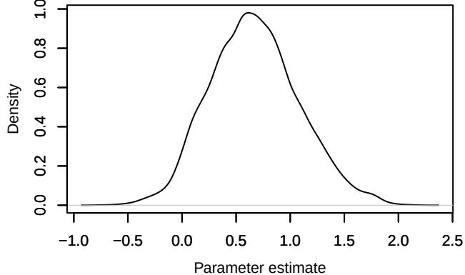
Density – betaISLAND_a[7]
