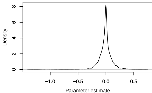
Density – betaISLAND_b[8]
