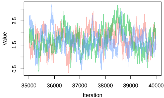
Trace – betaISLAND_a[4]
