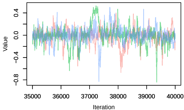
Trace – betaISLAND_b[2]
