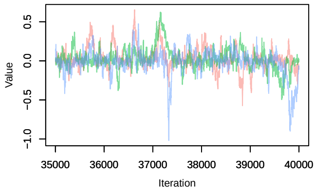
Trace – betaISLAND_b[7]
