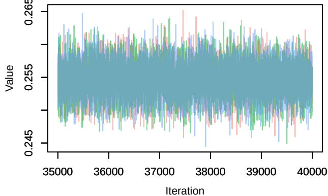
Trace – mean.p
