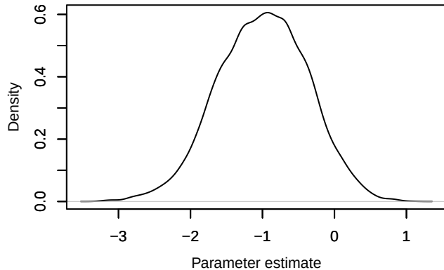
Density – betaISLAND_a[1]
