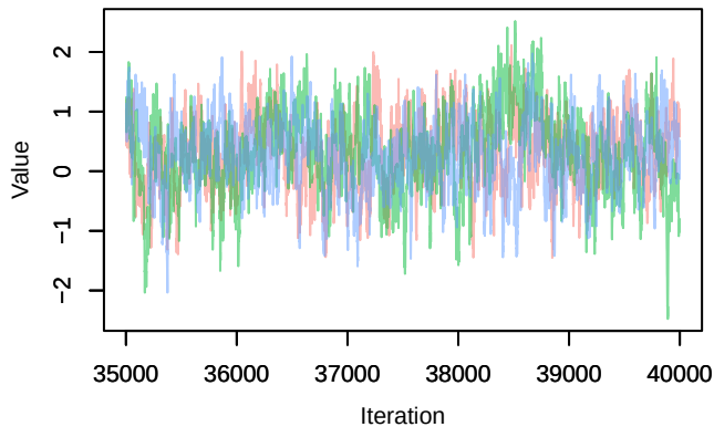
Trace – betaISLAND_a[6]
