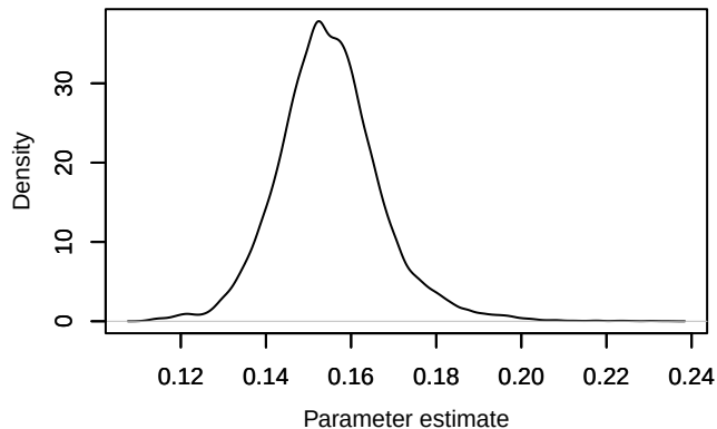
Density – betaISLAND_a[1]
