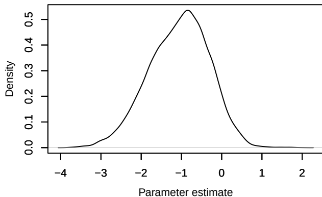
Density – betaISLAND_b[1]
