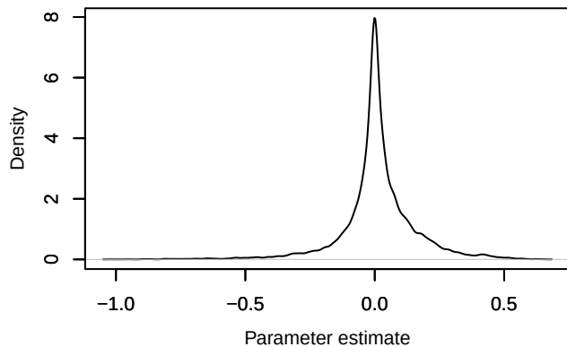
Density – betaISLAND_b[7]
