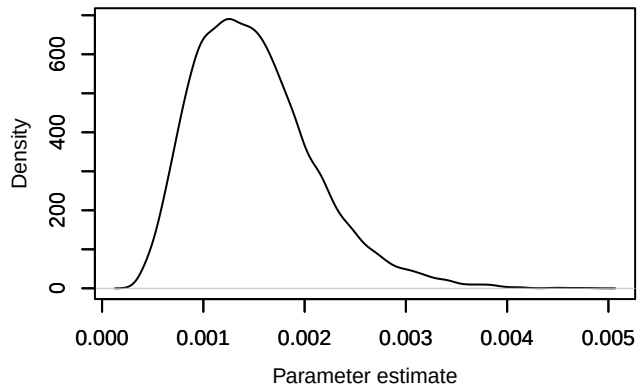
Density – b
