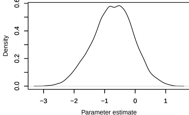
Density – betaISLAND_a[7]
