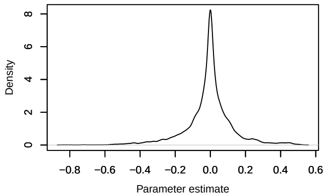
Density – betaISLAND_b[2]
