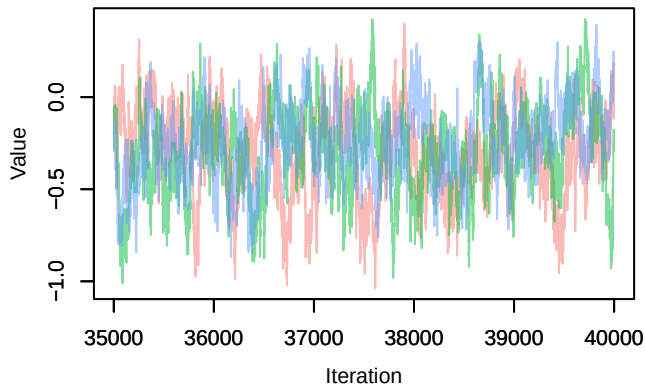
Trace – betaSEX[2]
