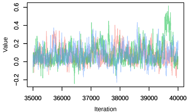
Trace – betaISLAND_b[4]
