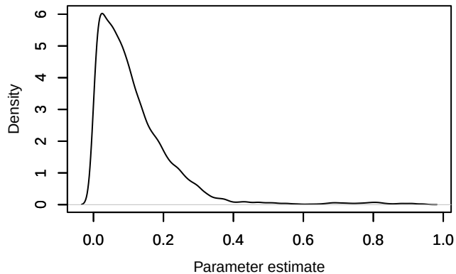
Density – sigma_b_island
