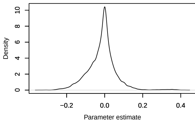
Density – betaISLAND_b[4]
