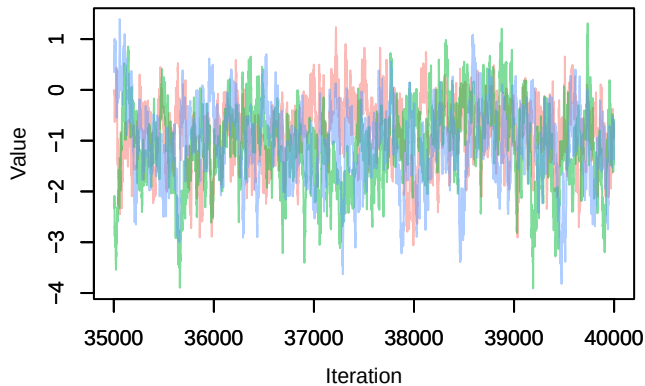
Trace – betaISLAND_a[3]
