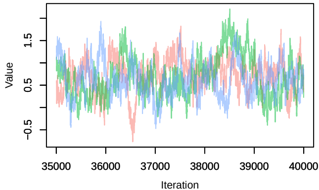
Trace – betaISLAND_a[7]
