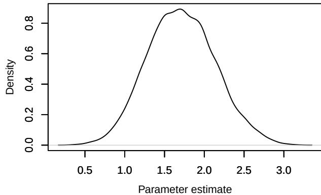
Density – betaISLAND_a[4]
