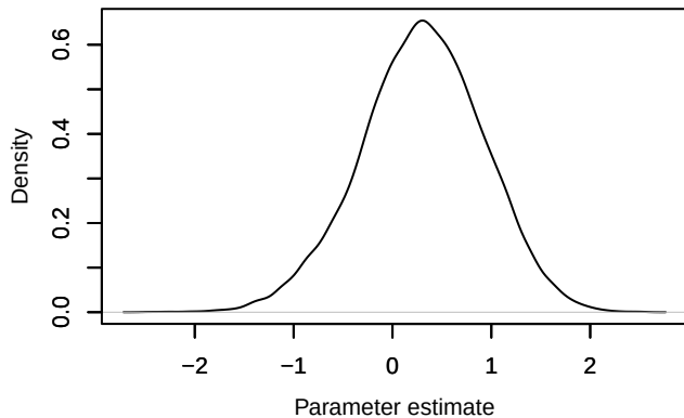
Density – betaISLAND_a[6]
