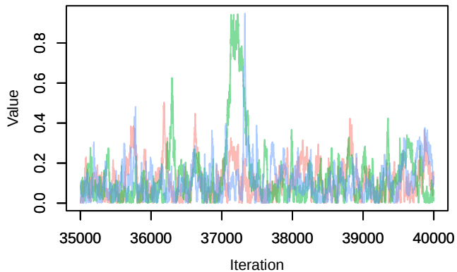
Trace – sigma_b_island
