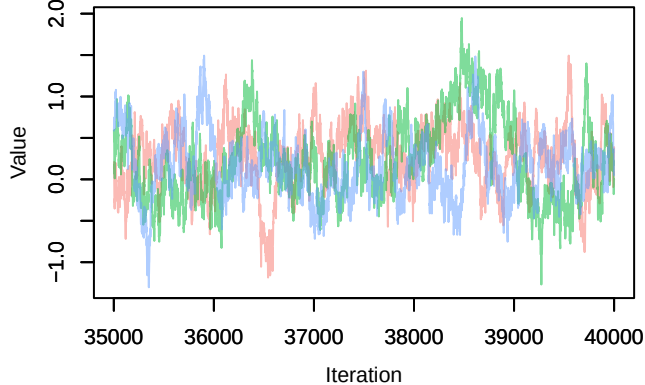
Trace – betaISLAND_a[4]
