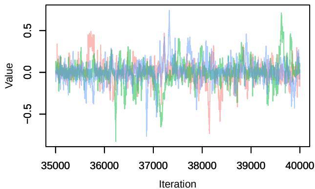
Trace – betaISLAND_b[5]
