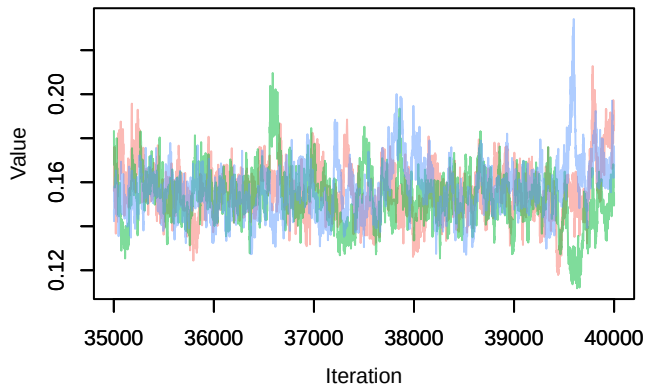
Trace – betaISLAND_a[1]
