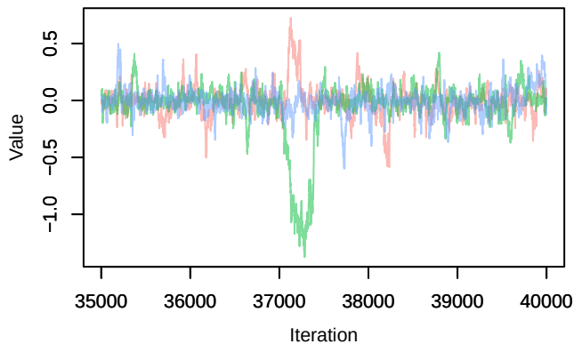
Trace – betaISLAND_b[8]
