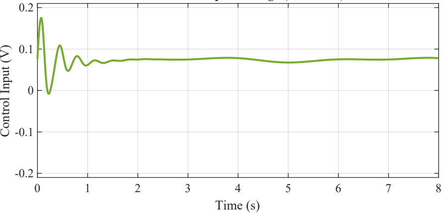
Controller Output Voltage (PID + FF)
